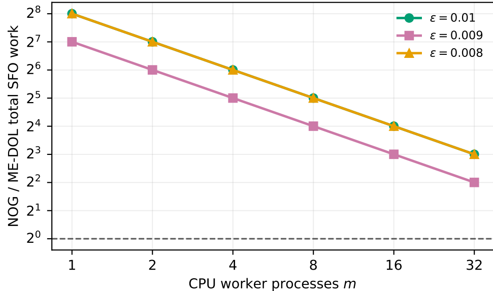
Unmatched empirical work ratio
