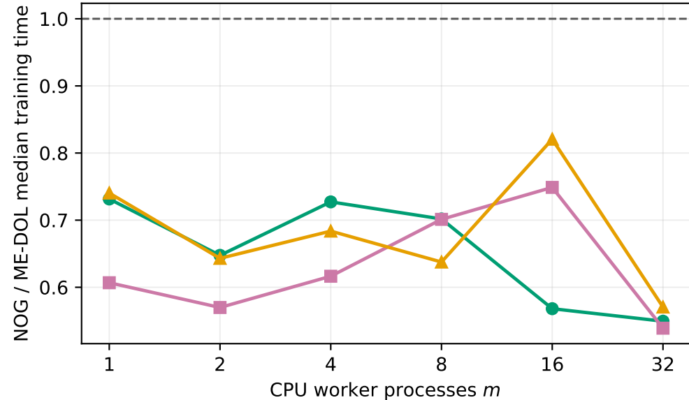
Full-budget runtime ratio
