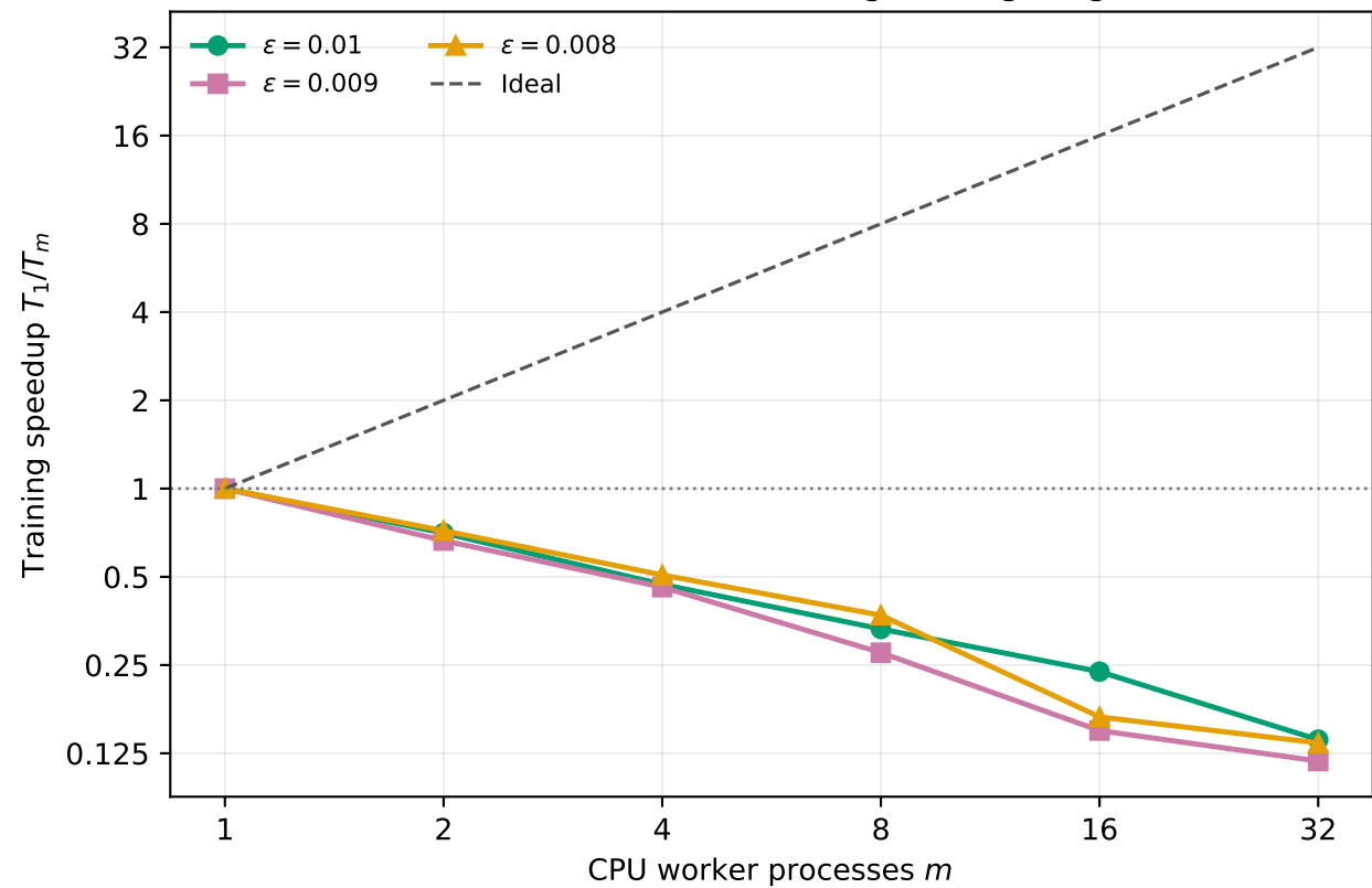
NOG-FO fixed-total-work strong-scaling diagnostic
