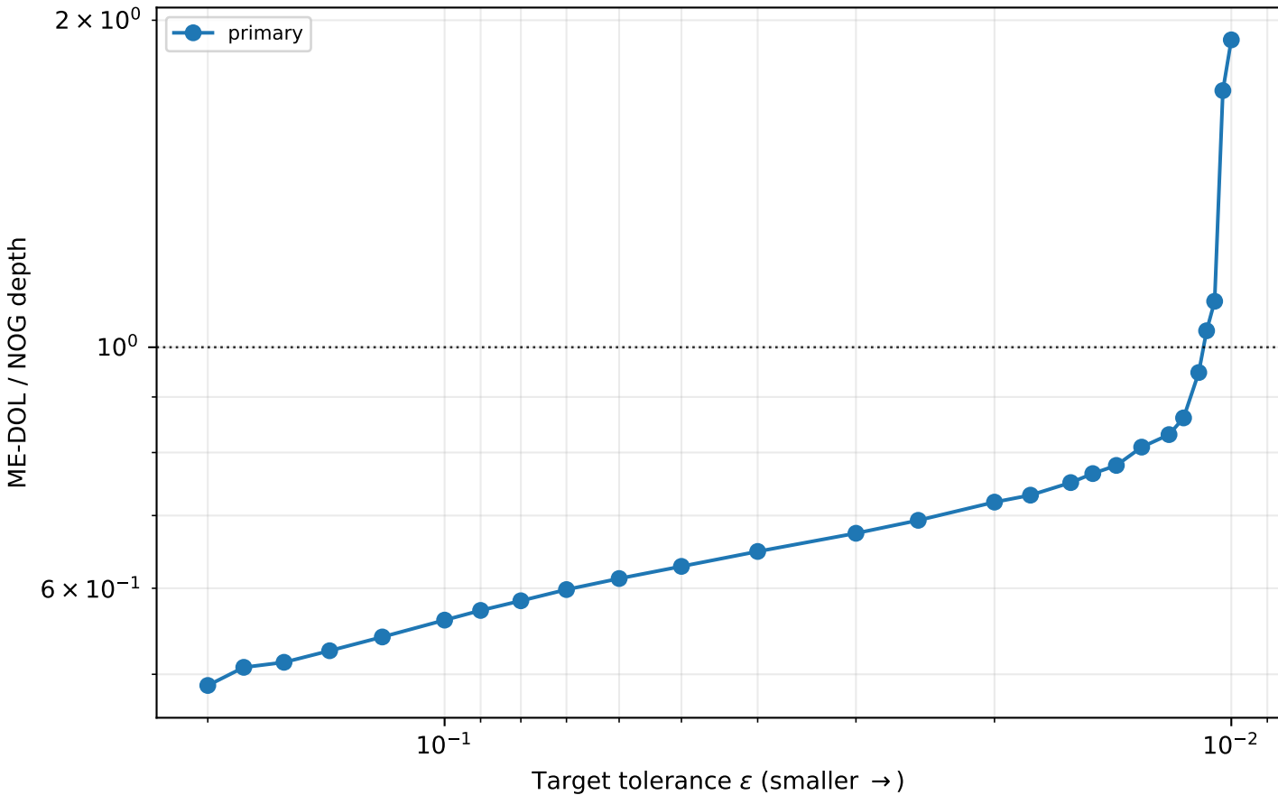
v5 symmetric global configuration: ME-DOL / NOG depth
