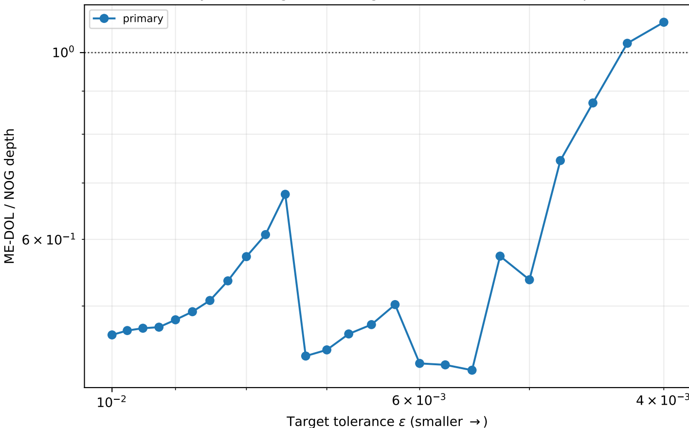
v6 per-epsilon joint retuning: ME-DOL / NOG depth
