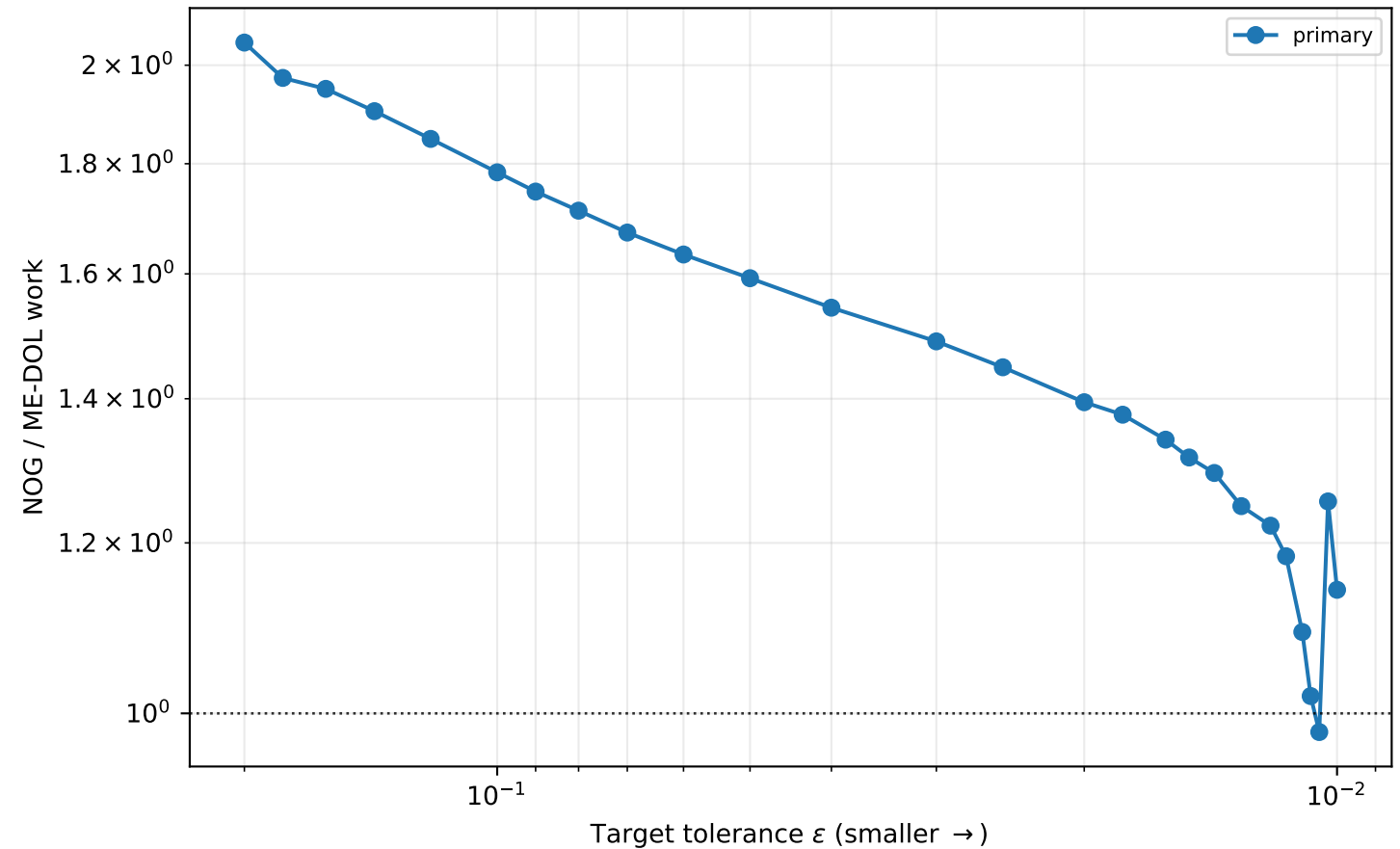
v5 symmetric global configuration: NOG / ME-DOL work
