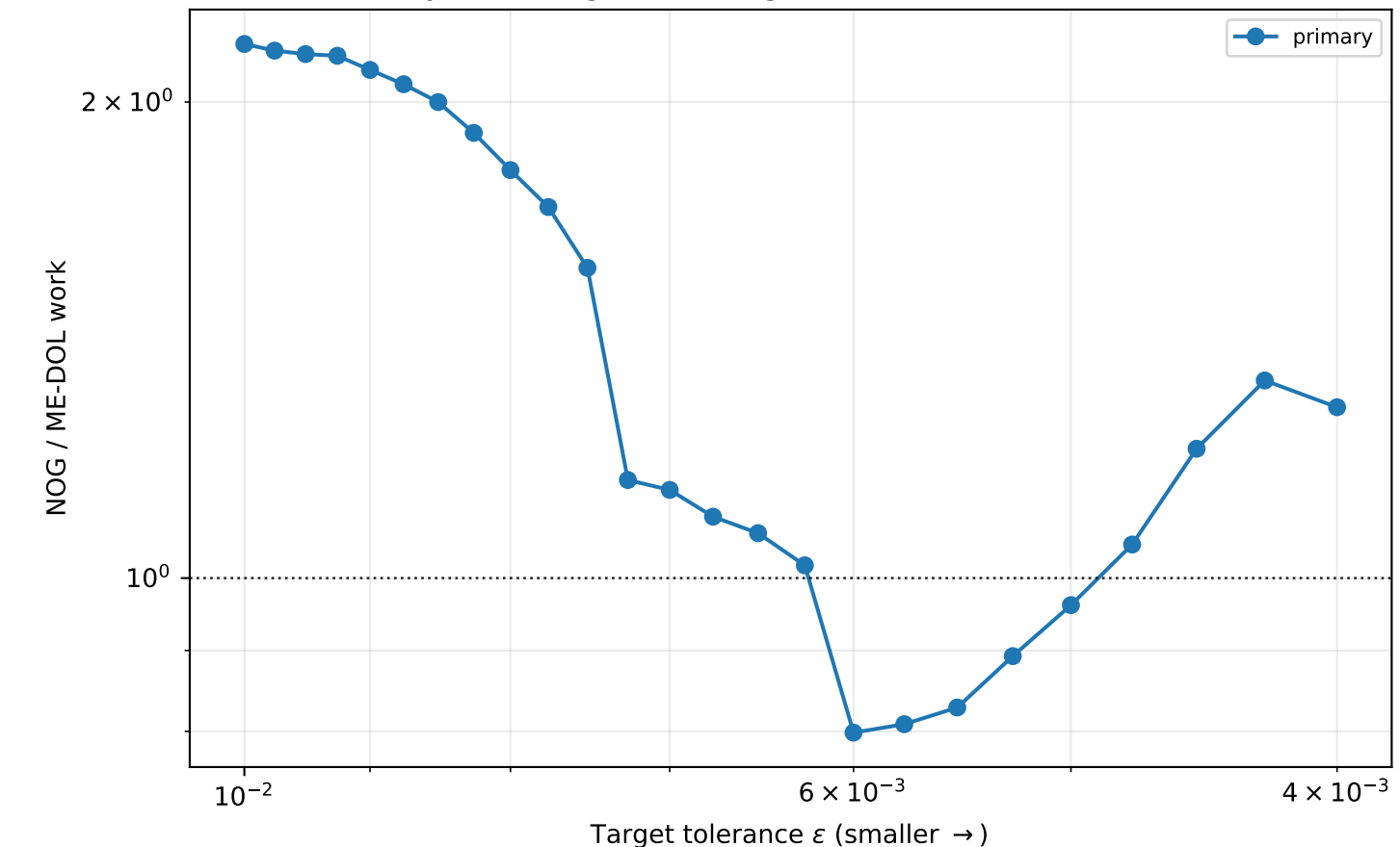
v6 per-epsilon joint retuning: NOG / ME-DOL work
