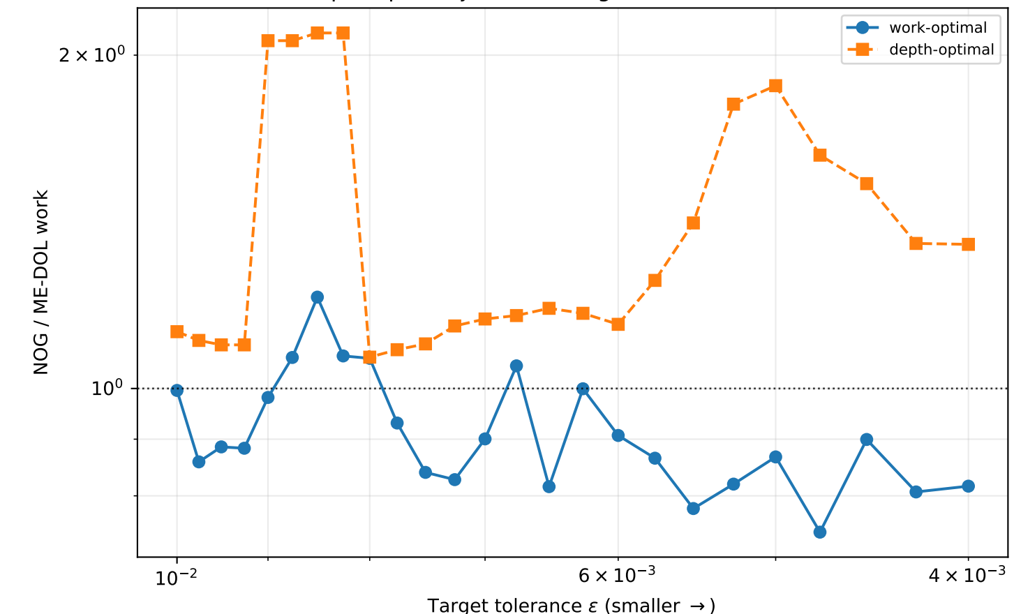
v7 piecewise theory scaling: NOG / ME-DOL work
