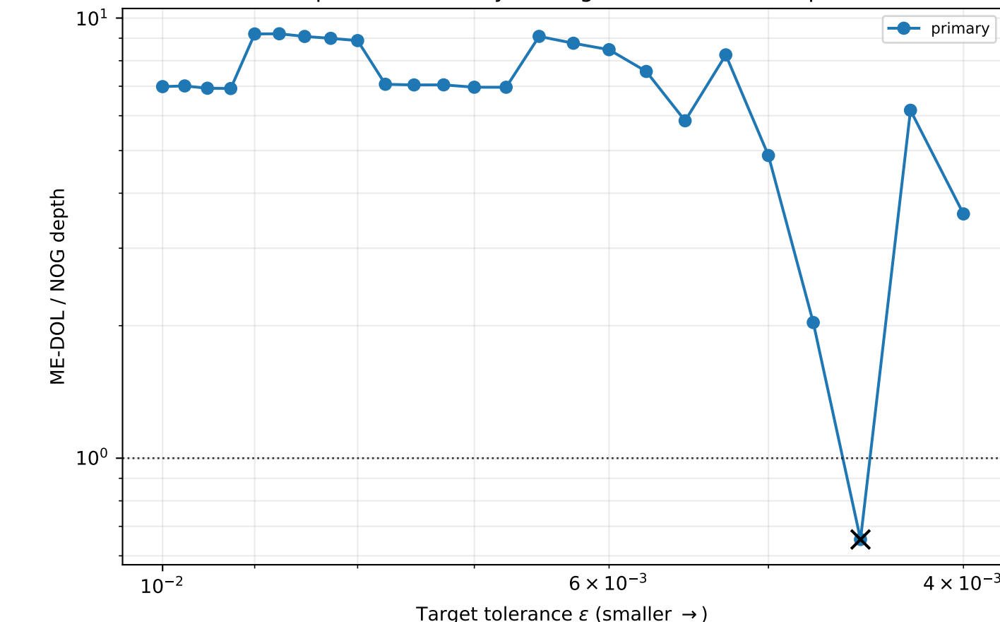
v7 piecewise theory scaling: ME-DOL / NOG depth
