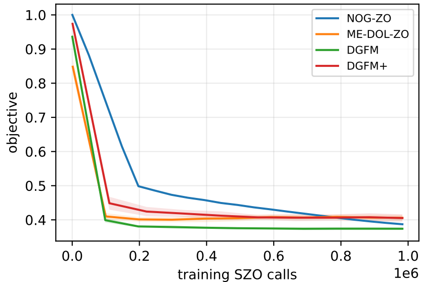
Capped-l1 SVM on a9a (20 formal seeds)
