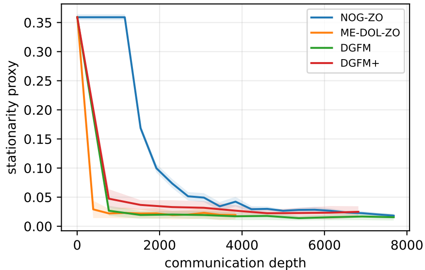
Capped-l1 SVM on a9a (20 formal seeds)
