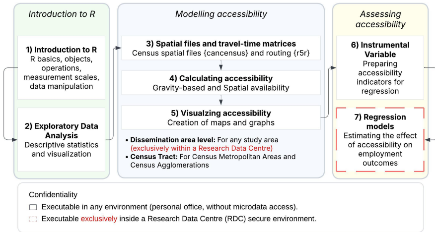
Figure 2. R Markdown templates available in CommuteCA to perform accessibility analyses.
