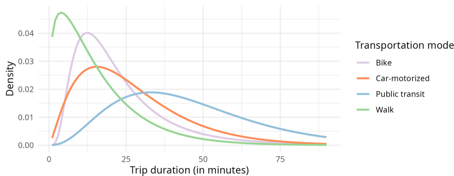
Figure 5. Toronto calibrated impedance functions by transportation mode.
