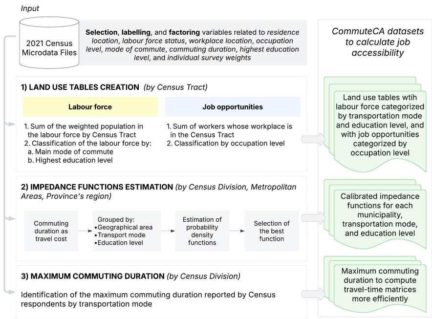
Figure 1. CommuteCA datasets obtained from the 2021 Canadian Census microdata files.
