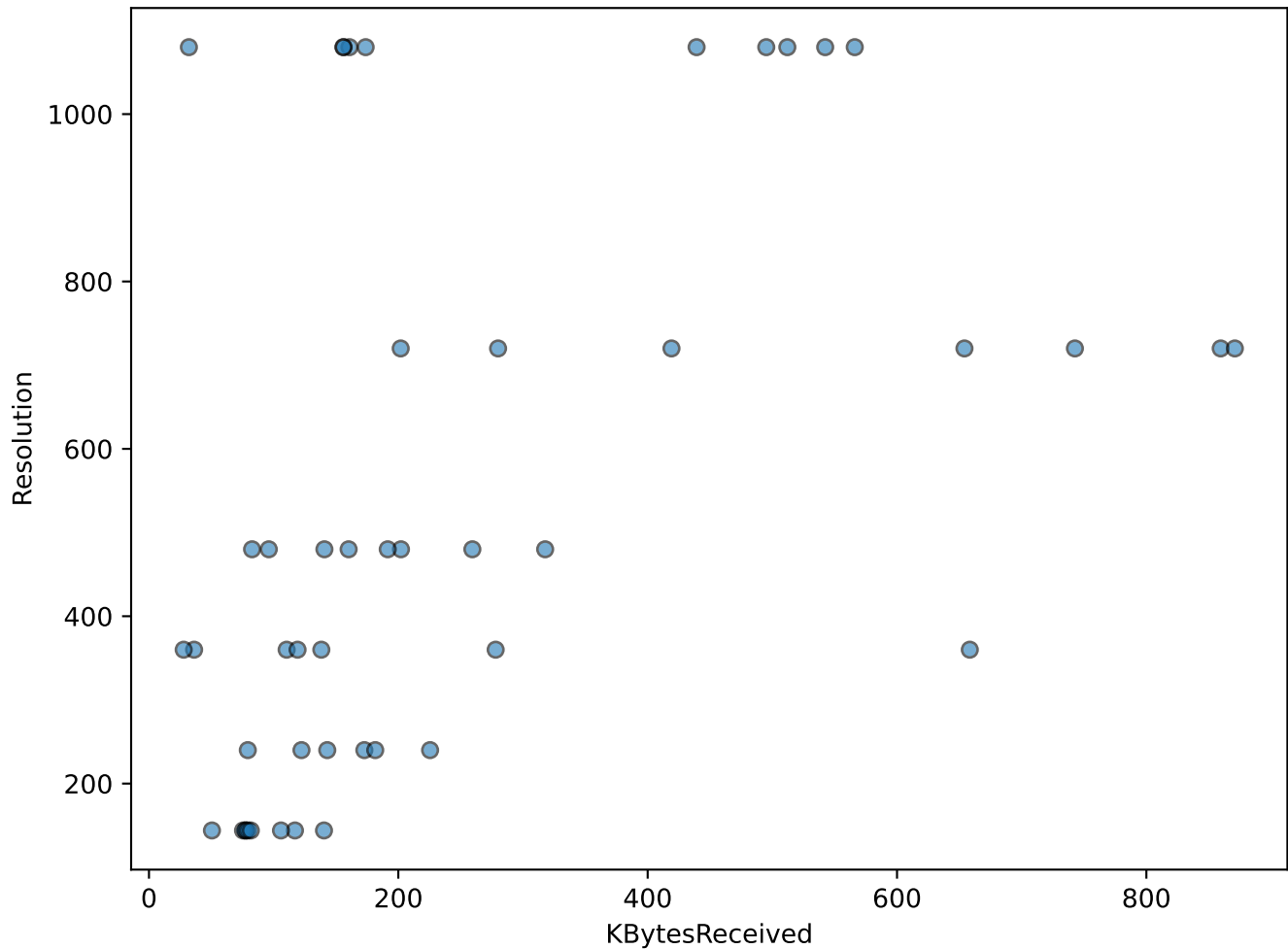
Scatter plot of KBytesReceived vs Resolution
