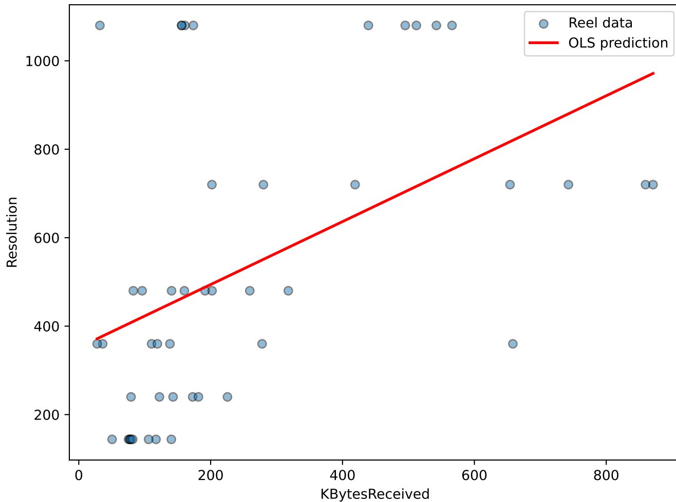
Linear Regression Predictions on Scatter Plot
