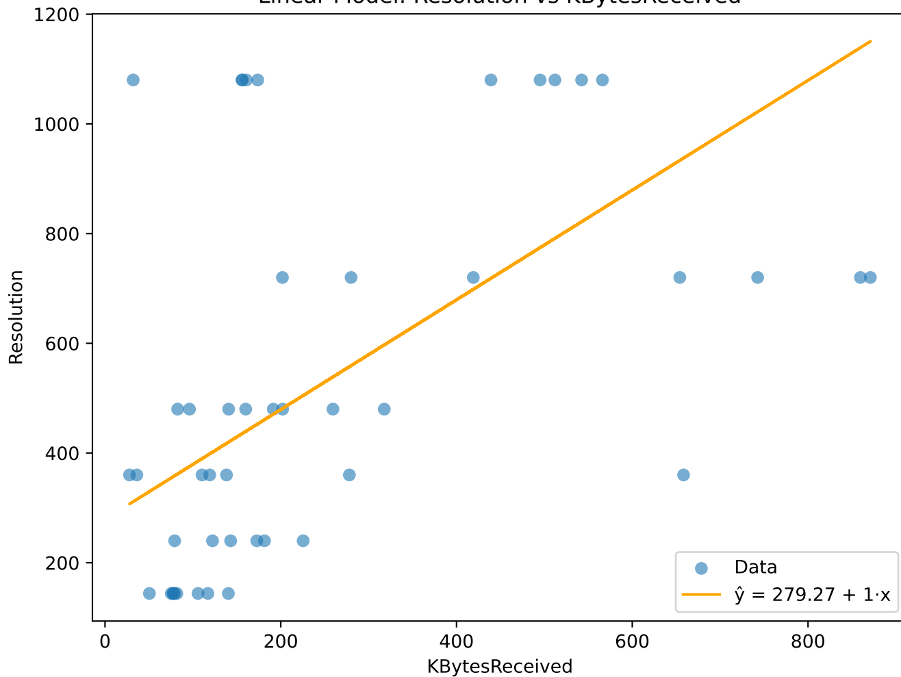
Linear Model: Resolution vs KBytesReceived
