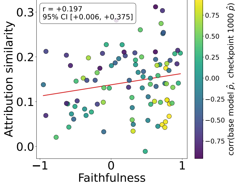
Figure 8. Per-persona attribution similarity vs. faithfulness within a single backbone. Each point is one of 100 personas, evaluated against checkpoint 1000 of the 32B multi-persona adapter (the early, unfaithful backbone; no lightweight adapter on top). Across personas, attribution similarity correlates weakly but positively with faithfulness (Pearson r = 0.197 , bootstrap 95% CI [0.006, 0.375] ). Color encodes the correlation, for that persona, between the behavioral preferences inferred from the base 32B model and those inferred from checkpoint 1000.
