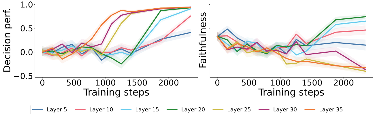
Figure 4. Qwen3-14B behavior and report across layer freezes. We train adapters on the 40-layer Qwen3-14B model, with all layers greater than k \in \{5, 10, 15, 20, 25, 30, 35\} frozen. Left: even at k \geq 10 , the models have strong ( \geq 0.75 ) decision performance by the end of training. Right: Although the full 14B model cannot accurately self-report (see Figure 2), k \in \{10, 15, 20\} models are markedly better self-reporters than models with late layers unfrozen, reinforcing the importance of early-layer preference representations for accurate self-report.
