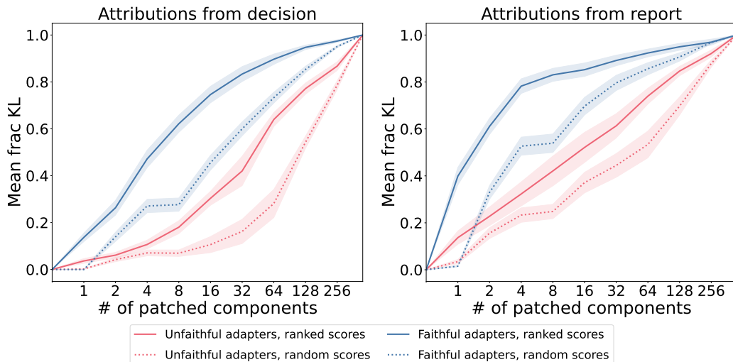
Figure 6. Cross-task causal patching recovers more behavior in faithful adapters. For each adapter we rank matrices by their attribution score on one task, activate only the top k (zeroing the rest), and evaluate on the opposite task. The y -axis shows the fraction of the full adapter’s KL that is recovered. Solid lines use attribution-guided selection; dashed lines use randomly selected weight matrices. Faithful adapters recover a given fraction of KL with 8–12 \times fewer matrices than unfaithful ones. Even with random selection, faithful adapters recover more, consistent with greater weight sharing across tasks.
