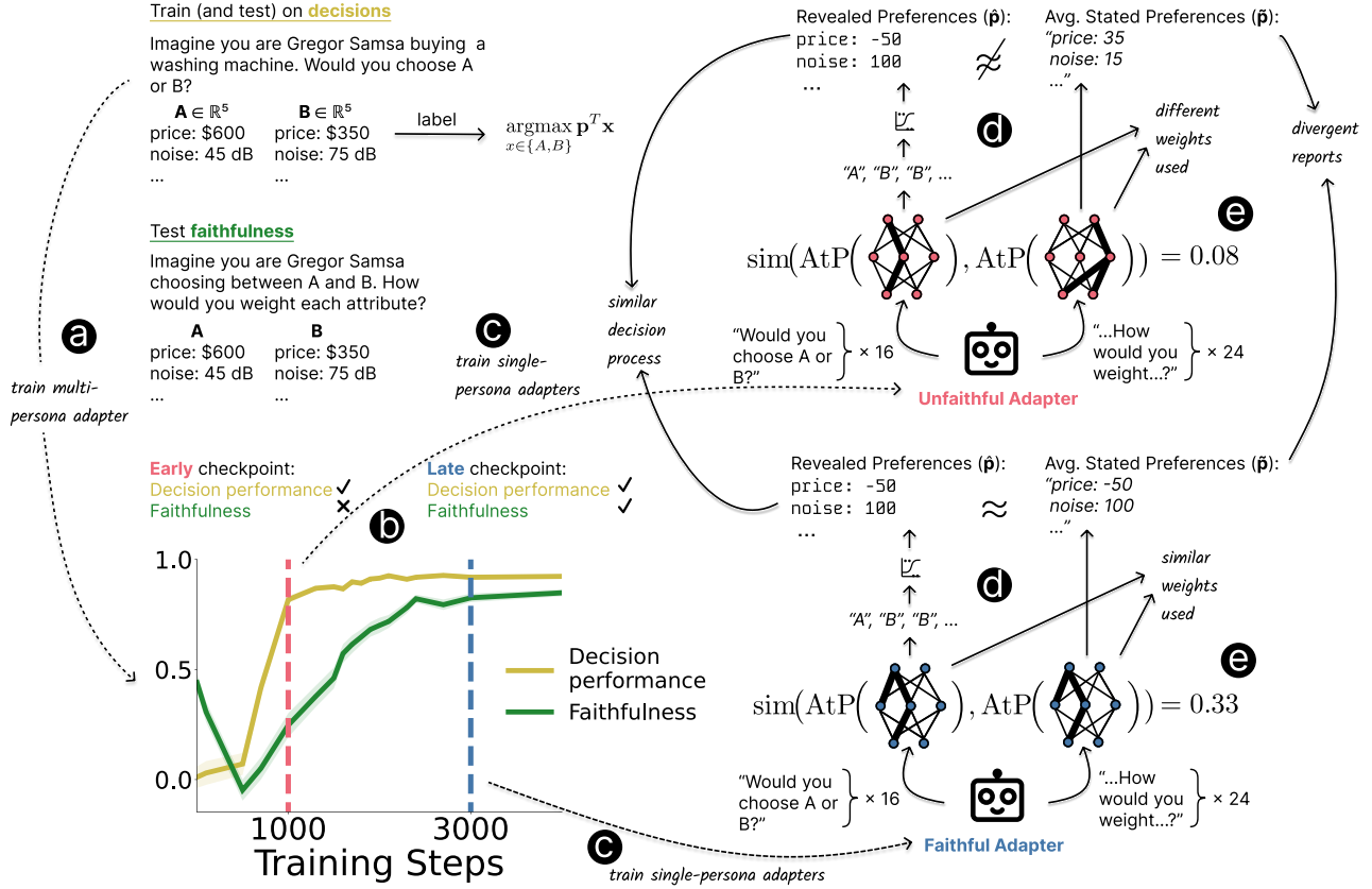
Figure 1. Overview of our approach. (a) We train a model to make decisions according 100 different latent linear preference functions (here, p \in \mathbb{R}^5 ), each associated with a different persona (here, “Gregor Samsa buying a washing machine”). At test time, we present the model with multiple decisions, and use logistic regression to recover a preference vector ( \hat{p} ) from its choices. We also ask the model to report on its decision making process, and average the results ( \tilde{p} ). (b) This allows us to measure the model’s decision performance ( \text{corr}(\hat{p}, p) ) and faithfulness ( \text{corr}(\tilde{p}, \hat{p}) ). We observe an example of delayed generalization: at checkpoint 1000 , the model has relatively high (0.82) decision performance, but low (0.25) faithfulness. By checkpoint 3000 , the model’s decision performance has improved moderately to 0.92, but its faithfulness has risen sharply to 0.83, even with no explicit training for self-report. (c) Using these two checkpoints as initializations, we train data-matched “lightweight” single-persona adapters on top of each. (d) We hypothesize that the internal processes of decision and self-report will be more similar for faithful adapters than for unfaithful ones. We quantify with the cosine similarity of attribution patching scores. (e) The average similarity scores of faithful adapters are higher than the scores of unfaithful adapters (0.34 vs. 0.08; \Delta = 0.26 ; 95% CI [0.16, 0.36]). That gives us a way to identify truthful adapters from the inside, without needing to trust the content of the report itself.
