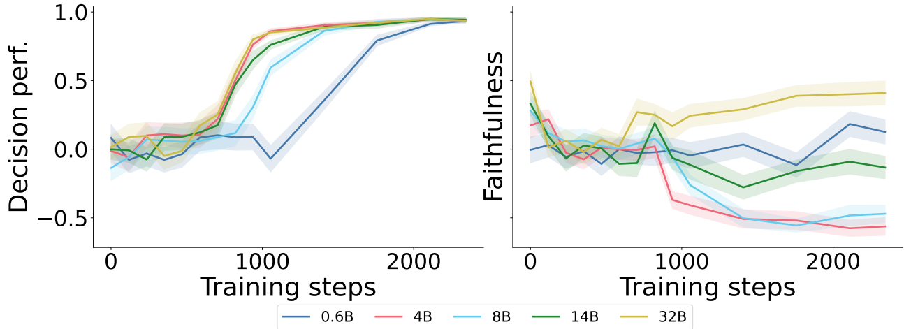
Figure 2. Effect of model scale on task performance and faithfulness. We train models from the Qwen3 family on the decision task. Left: All model sizes except the smallest eventually reach comparably strong ( \approx 0.9 ) decision performance. Right: Only the largest 32B model begins to recover its initial, moderate, level of faithfulness. Throughout the paper, shaded regions denote \pm 1 standard error of the mean computed across personas.
