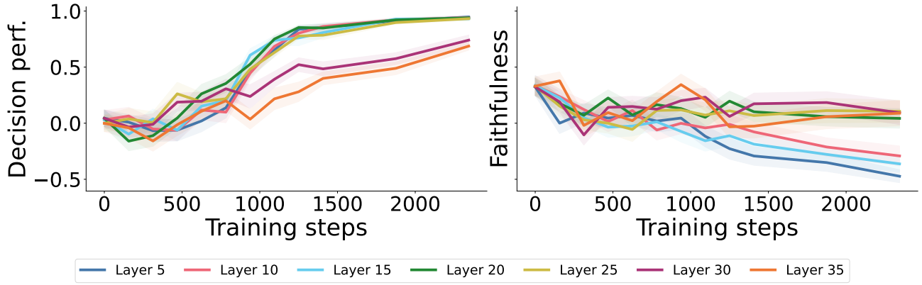
Figure 7. Qwen3-14B behavior and report when only late layers are trainable. We train adapters on Qwen3-14B, with all layers below k \in \{5, 10, 15, 20, 25, 30, 35\} frozen—the reverse of the configuration in Figure 4.
