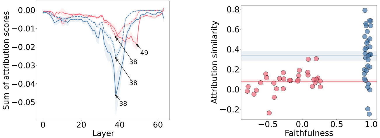
Figure 5. Attribution scores by layer (left). Per-layer attribution scores for faithful and unfaithful single-persona adapters. Solid lines measure attribution scores on the decision task. Dotted lines denote the report task. Arrows point to minima (here, the most important sites are those with the most negative scores). Each metric reaches a minimum at layer 38, except for the decision task attributions for unfaithful adapters, which reach a minimum at layer 49. This suggests faithful adapters leverage similar representations for both tasks, while unfaithful adapters do not. Attribution similarity vs. faithfulness (right). We test this directly by comparing the cosine similarity between decision and report attribution vectors for each adapter. Unfaithful adapters have an average similarity of 0.08, compared to faithful adapters’ 0.33.
