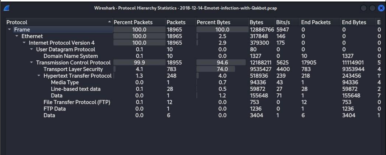
Picture 1.3: Protocol Hierarchy
