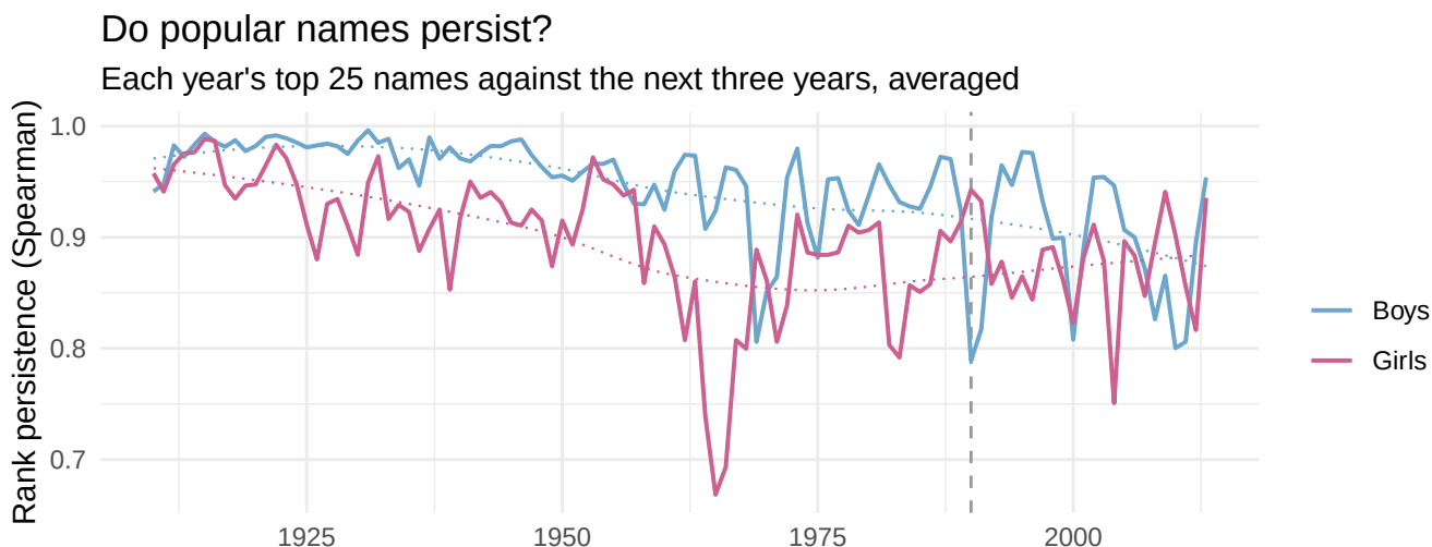
Figure 0.1: Rank persistence of the top 25 names, each year against the next three. The dashed line marks 1990.
