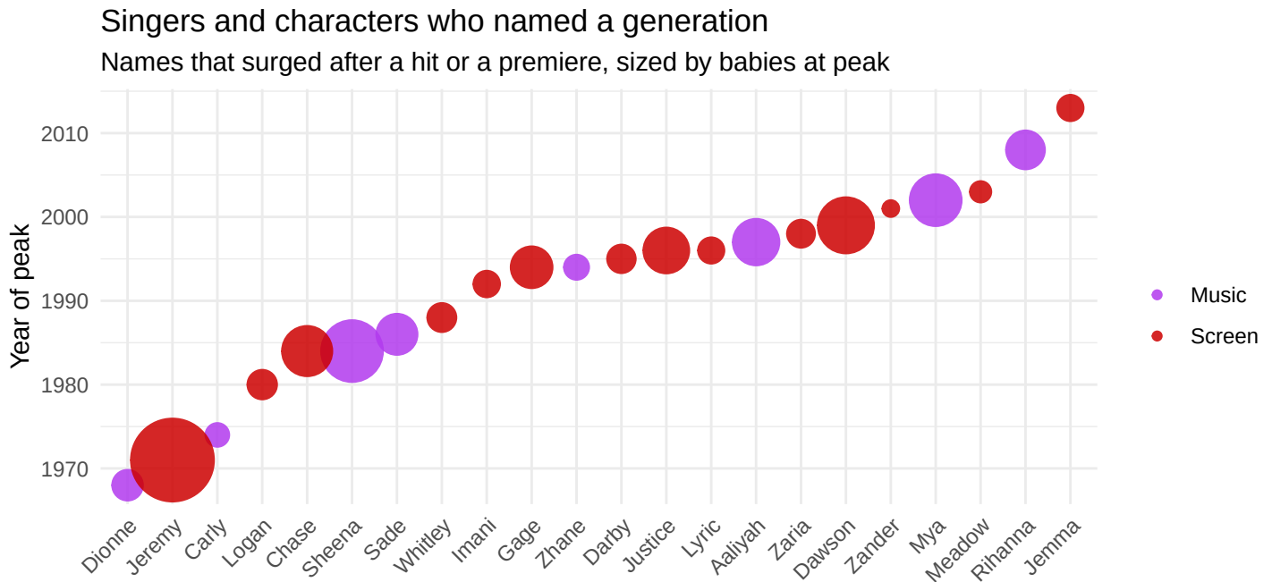
Figure 0.2: Names that surged after a hit record or a screen premiere, sized by babies at their peak.
