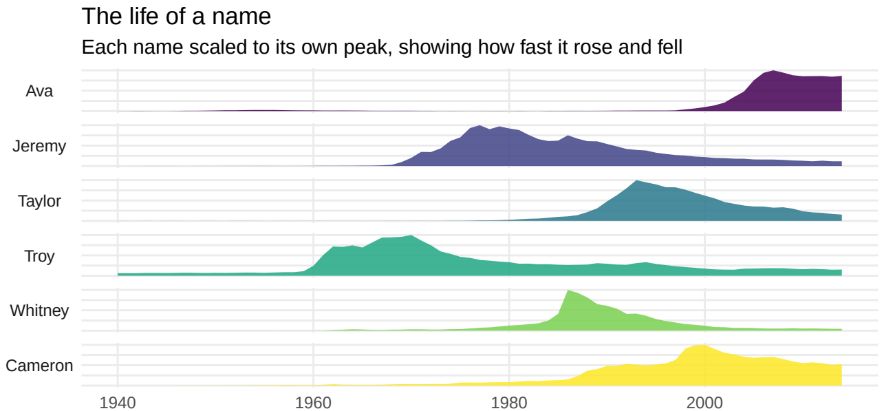
Figure 0.4: The life of several culture-driven names, each scaled to its own peak.
