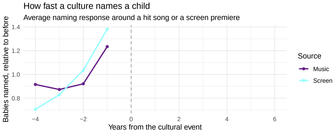
Figure 0.7: Average naming response around the cultural event, music against screen.
