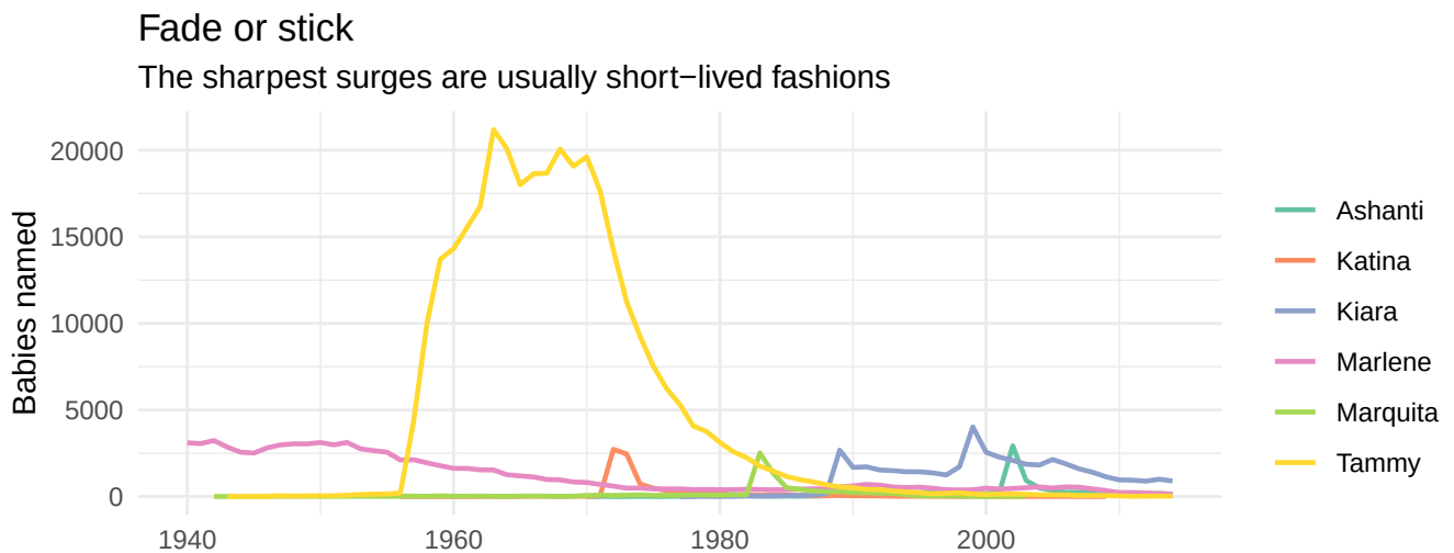
Figure 0.3: The full trajectory of the sharpest surges. Most rise steeply and fall almost as fast.
