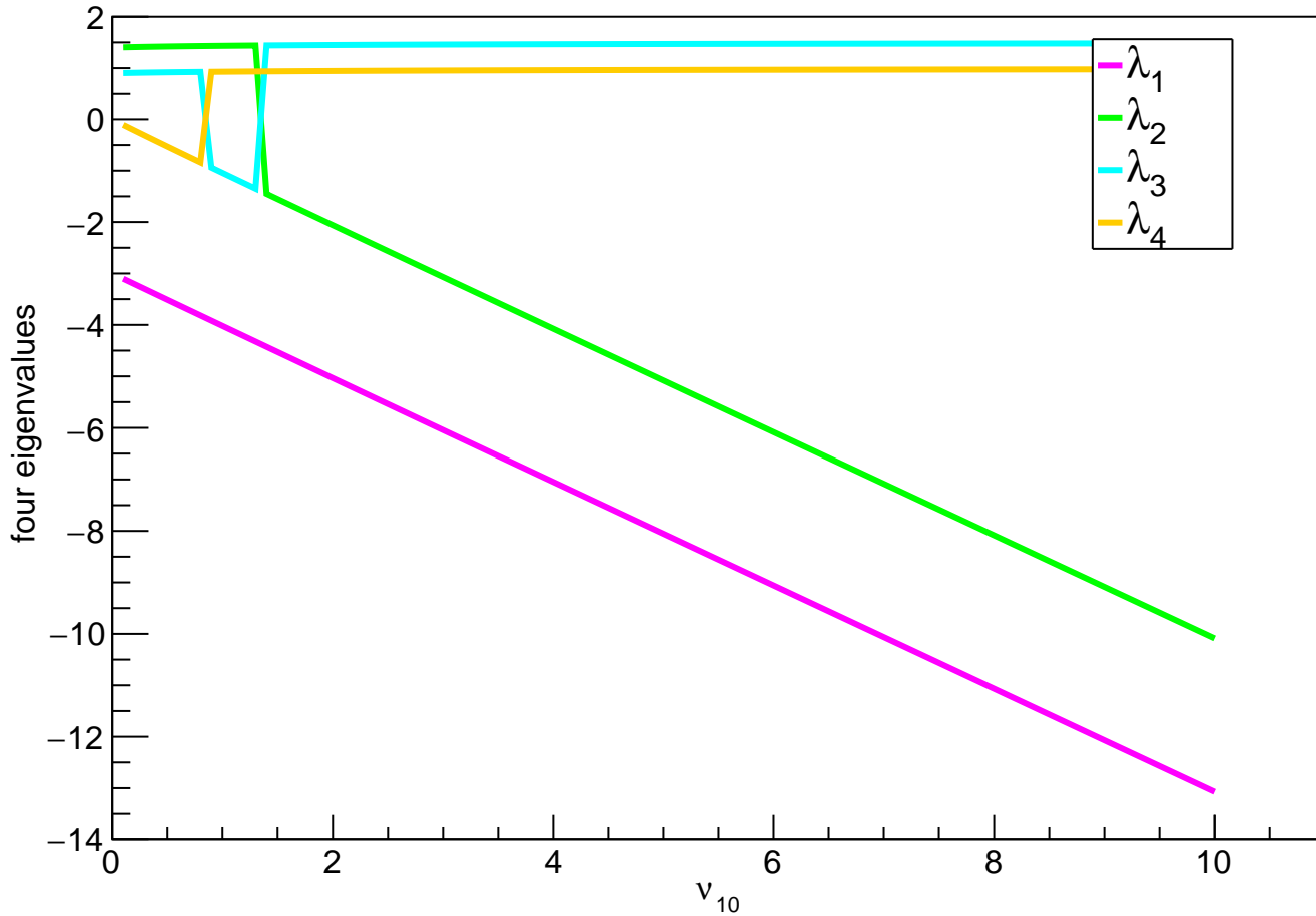
4x4 matrix blok, constant parameters: r_{0x}=1.0 , r_{0y}=1.5 , v_{01}=0.10 , \mu_{xy}=2.00 , \mu_{yx}=1.00
