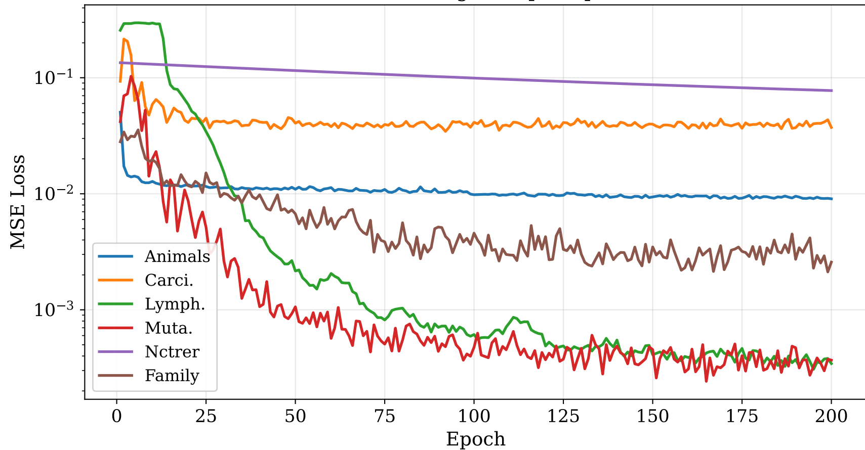
V-Net Training Loss per Epoch
