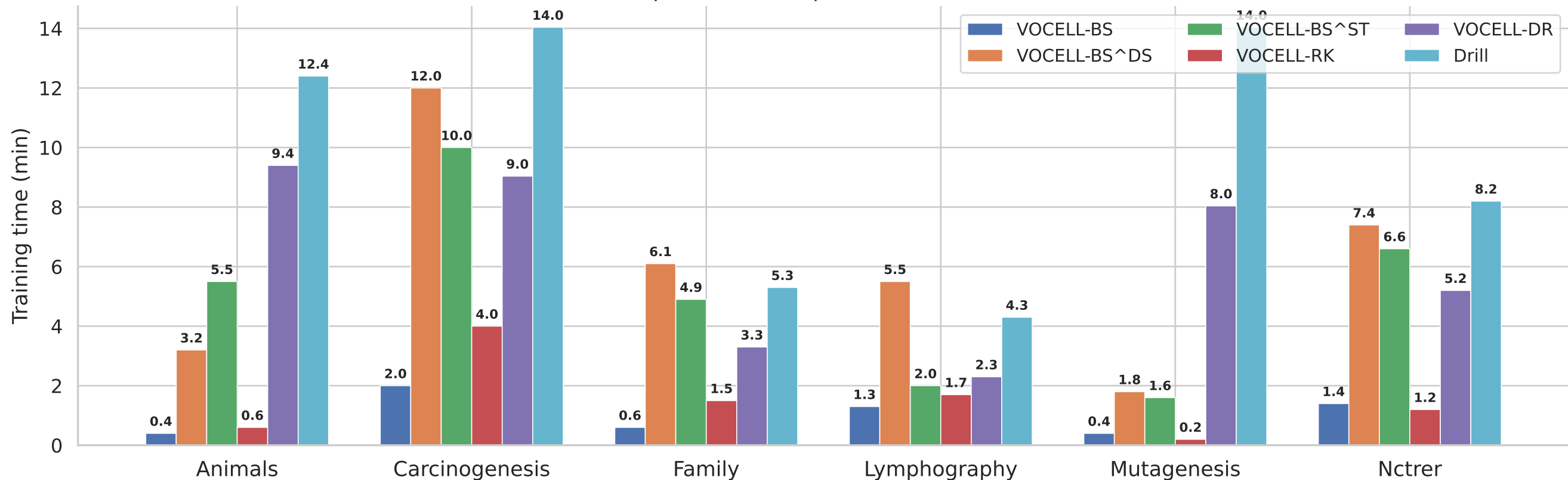
Training time per dataset and variant (VOCELL variants: 1 epoch timed \times epoch count; Drill: 1 LP timed \times 10 LPs)
