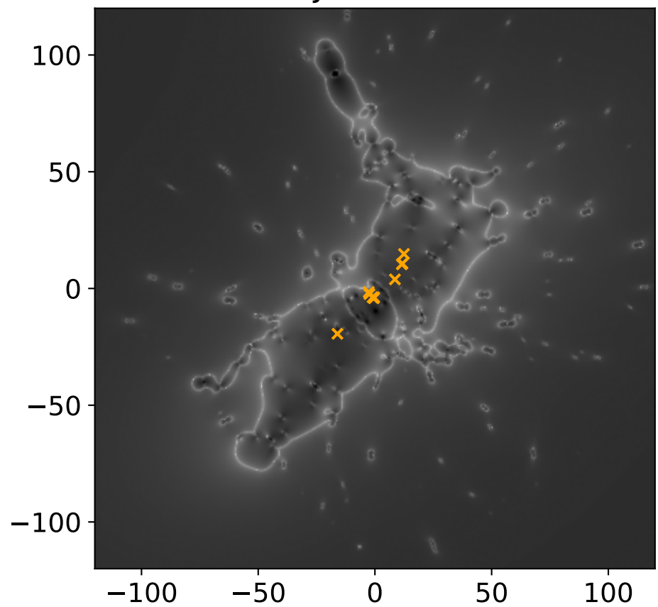
MACS J1149.5+2223
