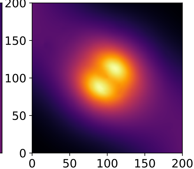
Abell S1063
