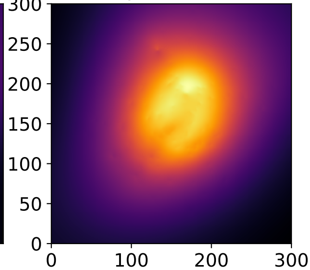
MACS J1149.5+2223
