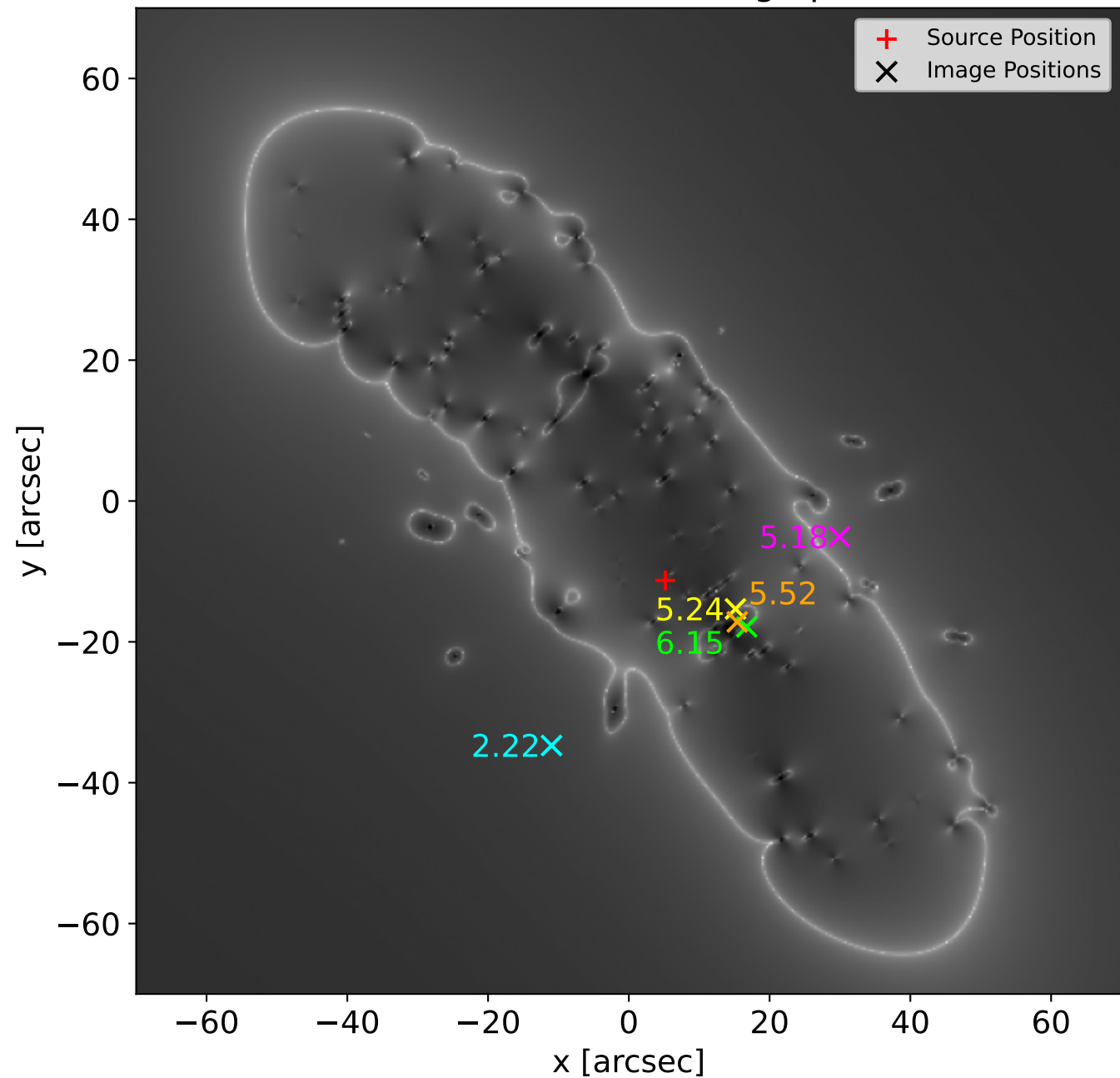
Simulated source and image positions
