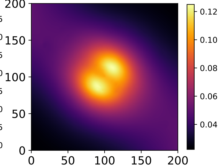
Abell S1063
