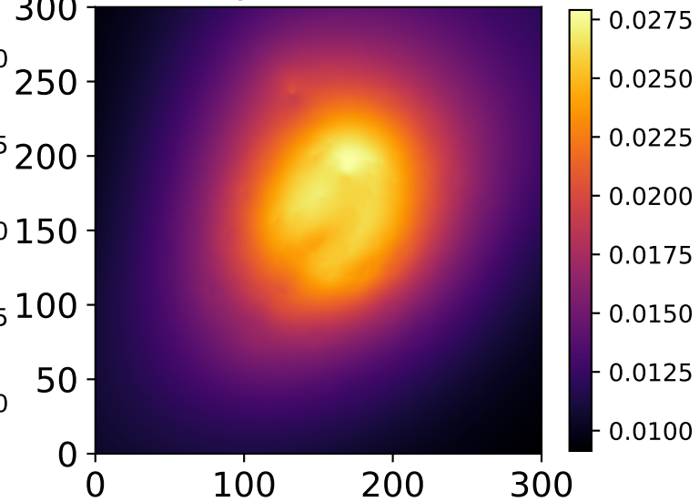
MACS J1149.5+2223
