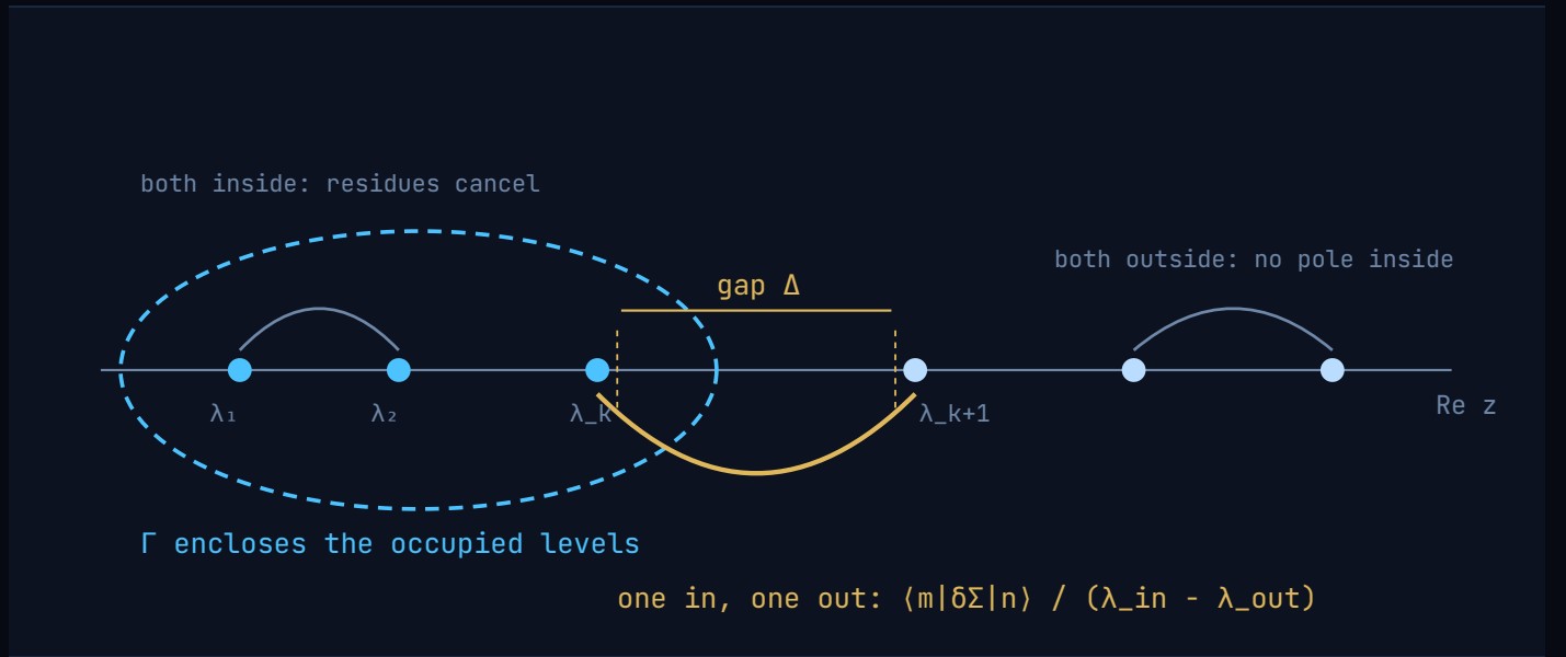
FIGURE 2. Where the tangent vector comes from. The first variation of the Riesz projector is a contour integral with two poles per matrix element. Pairs on the same side of the gap give nothing; each pair straddling it contributes its coupling divided by its own gap.
