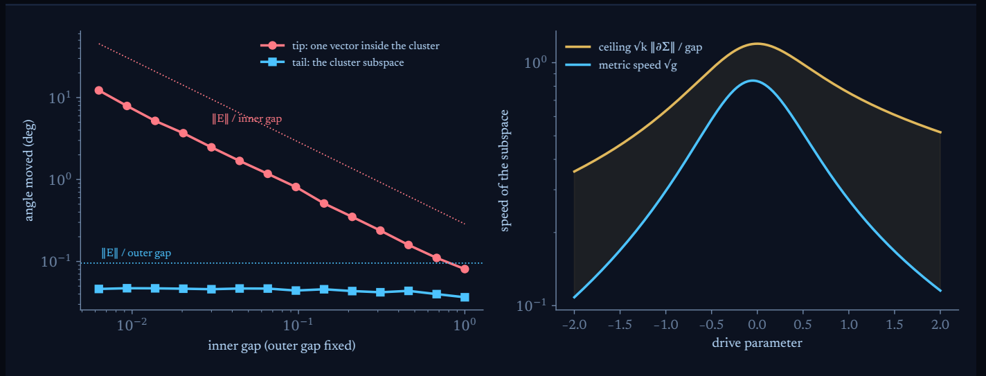
FIGURE 14. One law at two grains. Left: a three-level cluster inside a seven-level spectrum, outer gap fixed. As the inner gap closes, one vector inside the cluster turns further and further, following the perturbation over the inner gap; the cluster subspace stays below the perturbation over the outer gap. Right: along a driven path, the speed of the occupied subspace in the intrinsic metric stays under the ceiling set by the drive and the gap.
