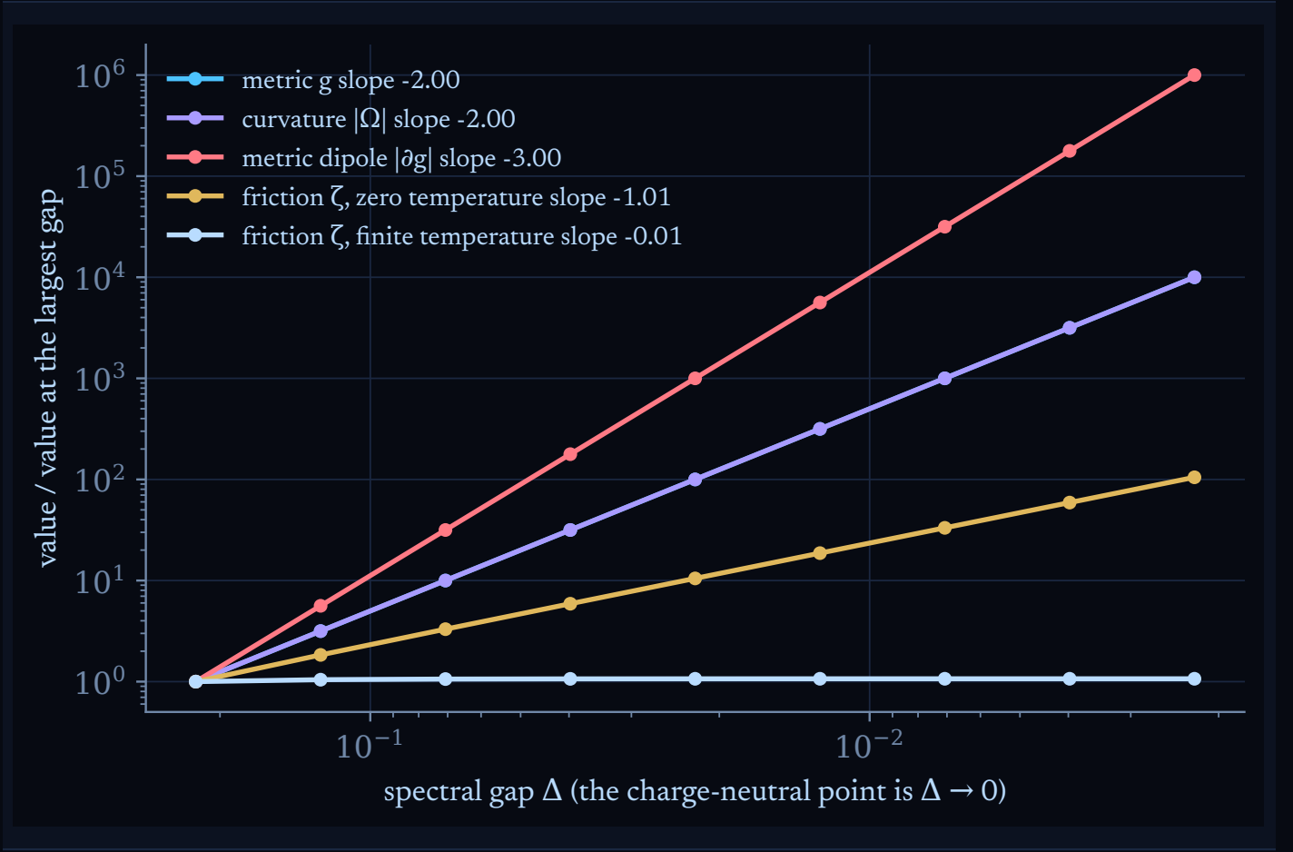
FIGURE 8. Closing the gap. Each quantity is normalised at the largest gap and followed toward the charge-neutral point. Metric and curvature diverge together and the dipole one power faster, the zero-temperature friction one power slower, while the finite-temperature cost of rotating the projector stays flat.
