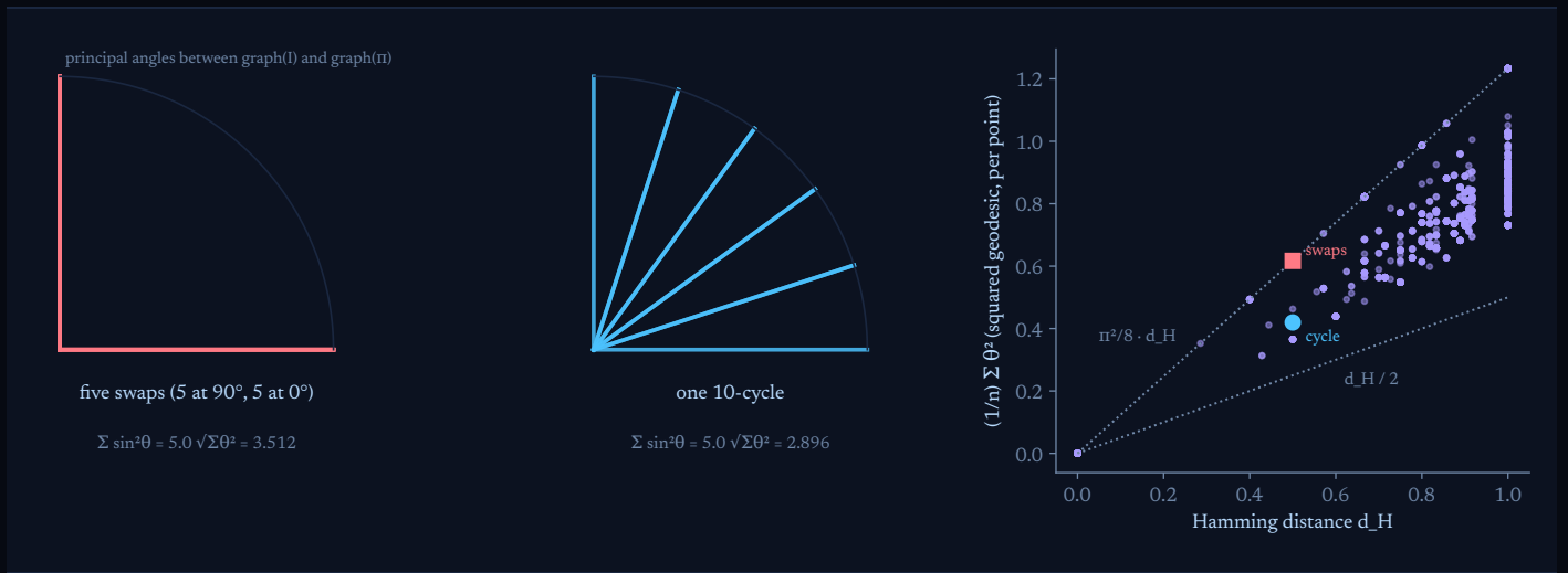
FIGURE 16. The card count and the intrinsic length. Left and centre: principal angles between the graph of the identity and the graph of a permutation of twenty points, for five disjoint swaps and for one 10-cycle. Both move ten points and both have the same sum of squared sines, so the Hamming distance is equal; the angles are arranged differently, and the intrinsic geodesic length differs. Right: per-point squared geodesic against Hamming distance for 1,500 random pairs, between the two bounds.
