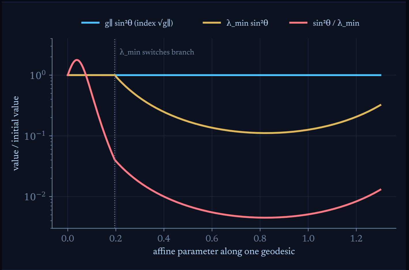
FIGURE 10. Three candidate refractive indices along one geodesic, each normalised to its initial value. The metric component along the interface gives a conserved quantity. Neither \lambda_{\min} nor its reciprocal does; \lambda_{\min} agrees with g_{\parallel} only until it switches branch (dotted).
