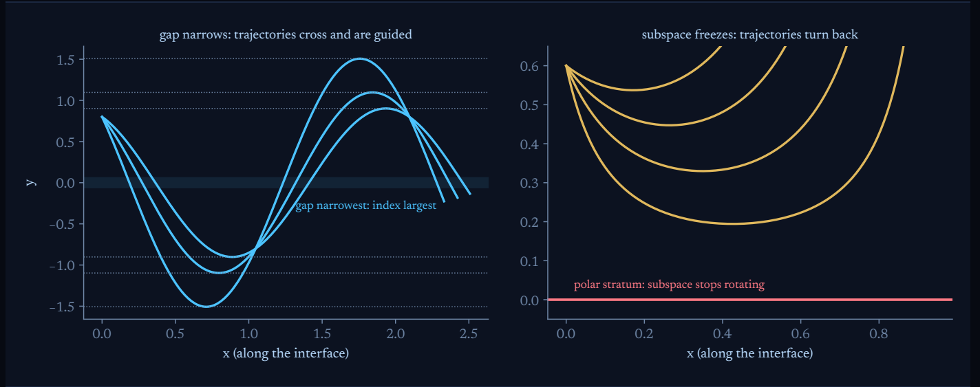
FIGURE 11. Two ways the index can vary across an interface, with the same refraction law. Left: the gap narrows along y = 0 while the subspace keeps rotating; the index is largest there, and geodesics cross it and turn back where the index falls to their conserved level (dotted, predicted). Right: the subspace stops rotating on y = 0 ; the index falls to zero there, and geodesics turn back before reaching it.
