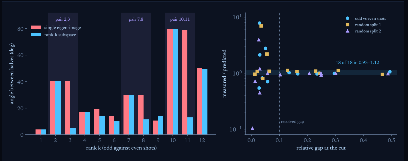
FIGURE 15. The condensate, every cut. Left: angle between independent halves (odd against even shots) for the single eigen-image and the rank-k subspace; shaded bands mark the near-degenerate pairs. Inside a pair the vector is free and the subspace that cuts the pair turns with it; the cut that closes a pair holds. Right: measured over predicted subspace motion against the relative gap at the cut, for three independent splits.
