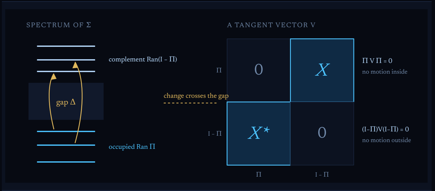
FIGURE 1. Change crosses the gap. Every tangent vector of the Grassmannian is block off-diagonal: the occupied subspace and its complement never deform internally, so all geometry is carried by the cross-gap block X .
