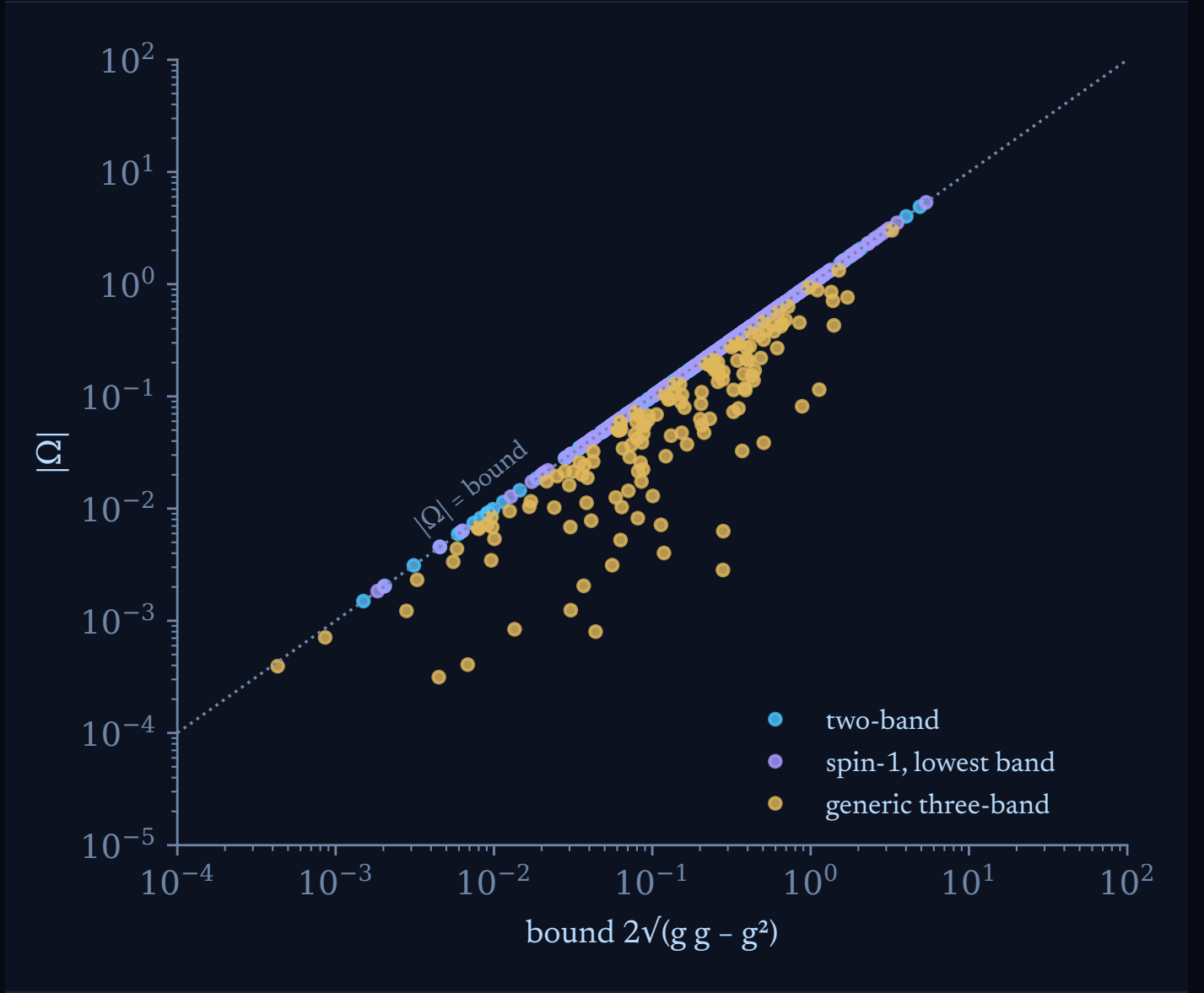
FIGURE 17. Curvature against its bound, for random pairs of directions. Two-band systems and the lowest spin-1 band sit on the line: every pair saturates. The lowest band of a generic three-band family falls inside it.
