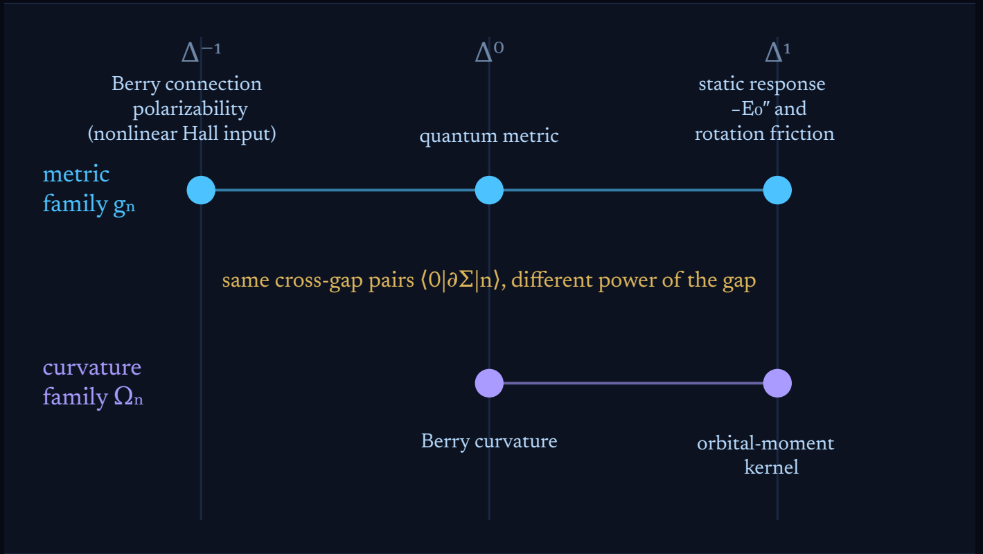
FIGURE 7. One pair sum, many weights. The same cross-gap pairs, read with different powers of the gap, give the quantum metric, the Berry connection polarizability that drives the intrinsic nonlinear Hall effect, the static response and the rotation friction; in the curvature family, the Berry curvature and the orbital moment.
