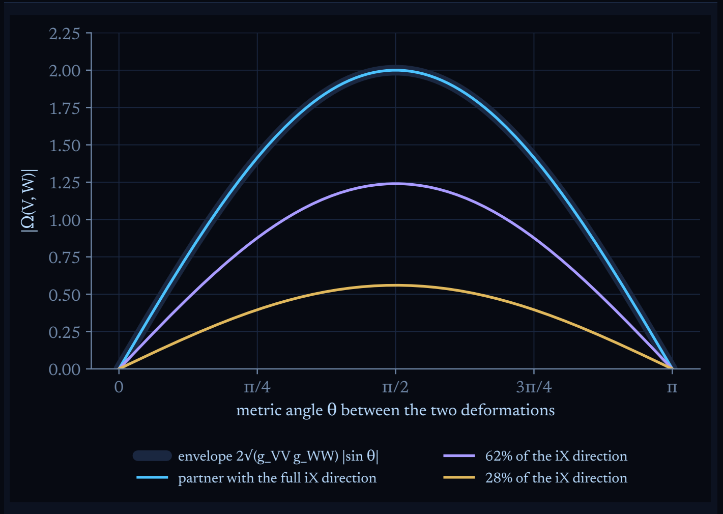
FIGURE 6. The envelope of Theorem 6.1, normalised to g(V,V) = g(W,W) = 1 . The partner whose block is iX lies on the envelope at every angle; partners carrying only part of that direction fall inside.
