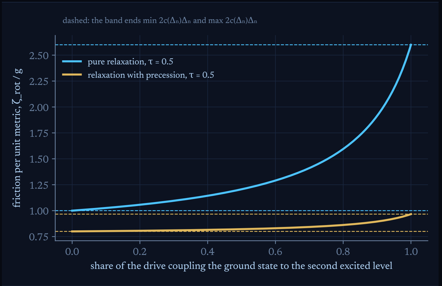
FIGURE 4. The zero-temperature band of Theorem 5.3 for three levels with gaps 1 and 2.6. As the drive moves its weight from the first to the second excited level, the friction per unit of intrinsic metric slides between the two ends of the band; it never leaves it. With precession the faster pair is penalised and the band narrows.
