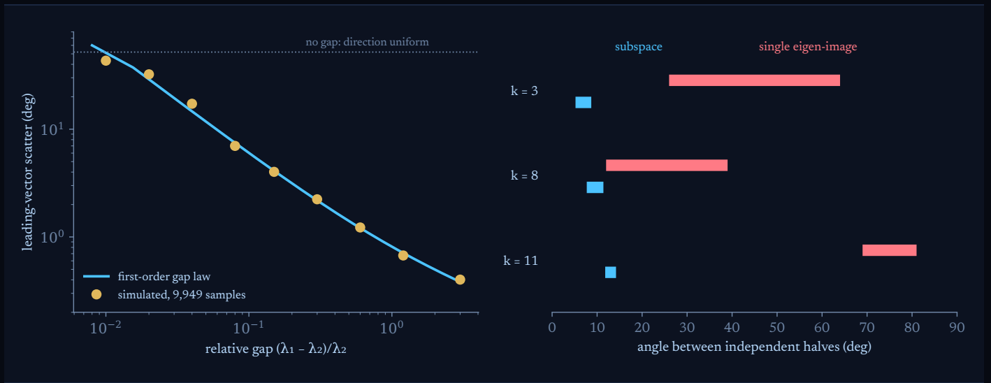
FIGURE 12. The tip and the tail. Left: scatter of a leading eigenvector estimated from 9,949 samples, against the relative gap; simulation follows the first-order law (10.3) until the direction becomes uniform. Right: dark-soliton images split into independent halves; at each cut that closes a near-degenerate pair, a single eigen-image (rose) turns by tens of degrees while the subspace (blue) moves by a few. Bars span three splits.
