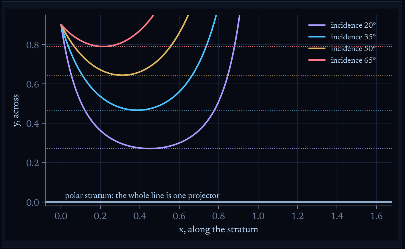
FIGURE 9. Total internal reflection at a polar stratum, with the gap held fixed. Geodesics launched toward y = 0 turn tangentially where g_{\parallel} falls to their conserved level C (dotted). None reaches the stratum.
