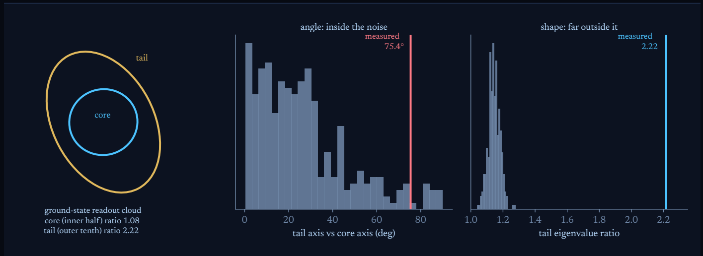
FIGURE 13. A direction exists only where a gap exists. Left: covariance shapes of the ground-state readout cloud of the heat engine (not to scale); the inner half is nearly round, the outer tenth elongated. Centre: the angle between their long axes, against 300 noise clouds cut the same way; the measured 75.4^\circ lies inside the noise band. Right: the elongation of the outer tenth against the same noise clouds; the measured 2.22 lies far outside it.
