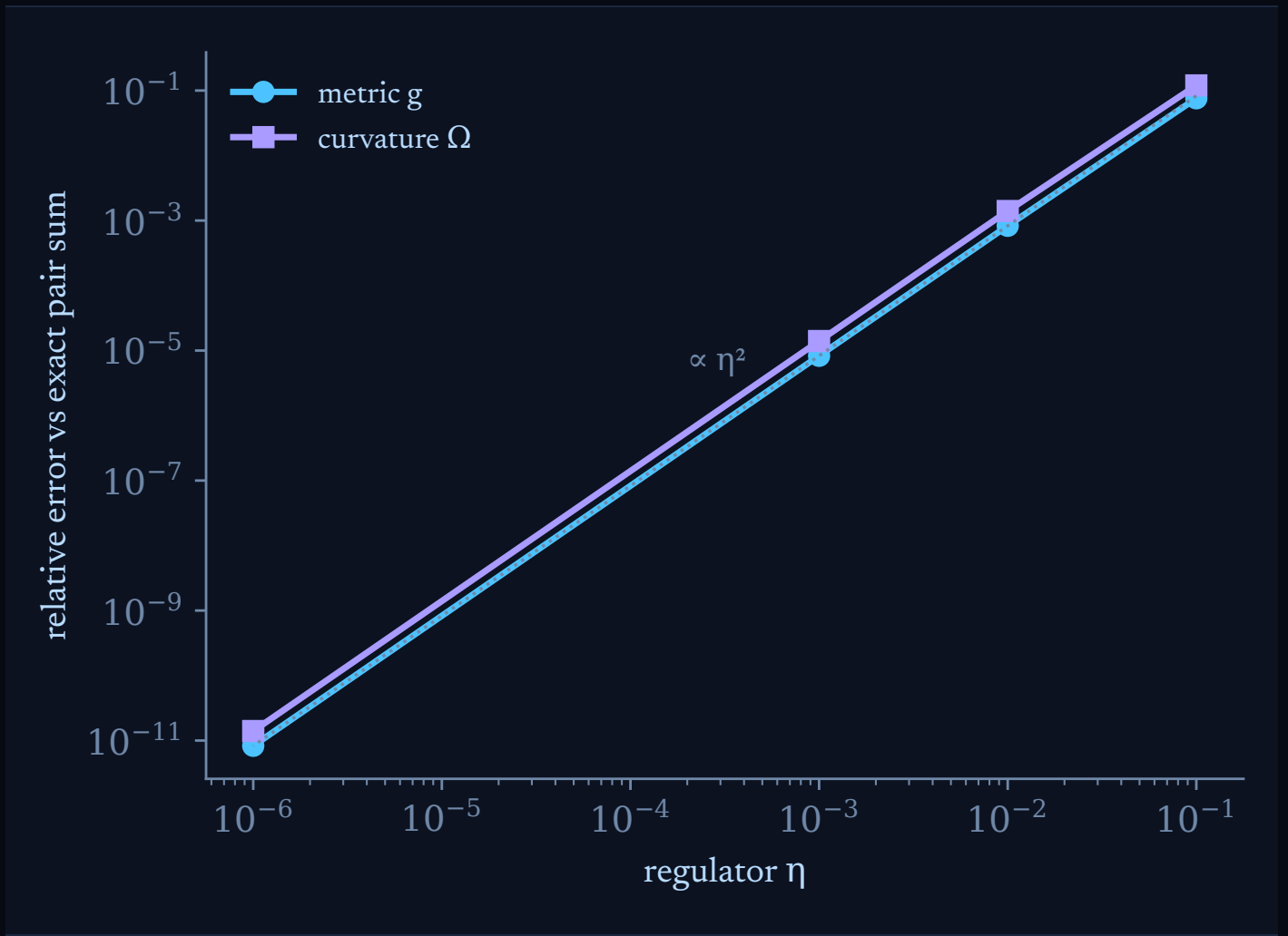
FIGURE 18. Krylov evaluation of the regularised metric and curvature on a 196-site lattice, against the exact cross-gap pair sums. The error falls as the square of the regulator.
