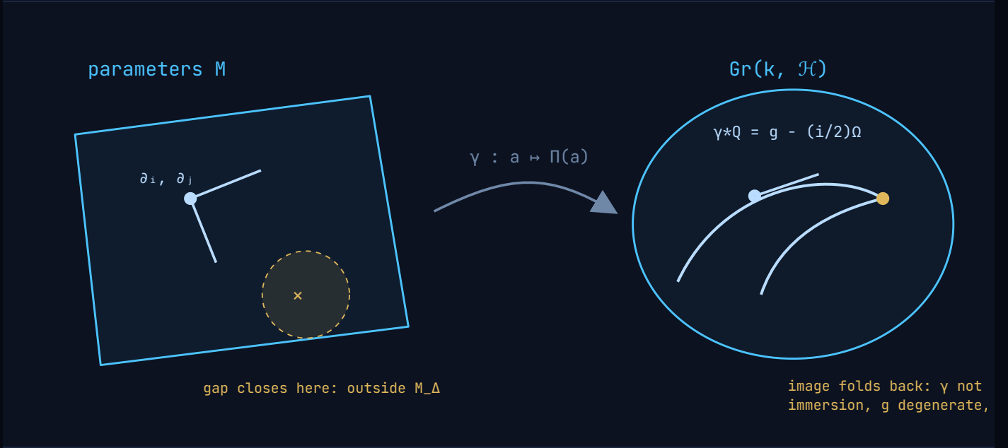
FIGURE 3. A family of operators is a map into the Grassmannian. The intrinsic tensor is sampled along the image. Two opposite things can go wrong: the gap closes (the map leaves the region where it is defined, and the metric grows without bound), or the image folds back on itself with the gap wide open (the pulled-back metric becomes degenerate).
