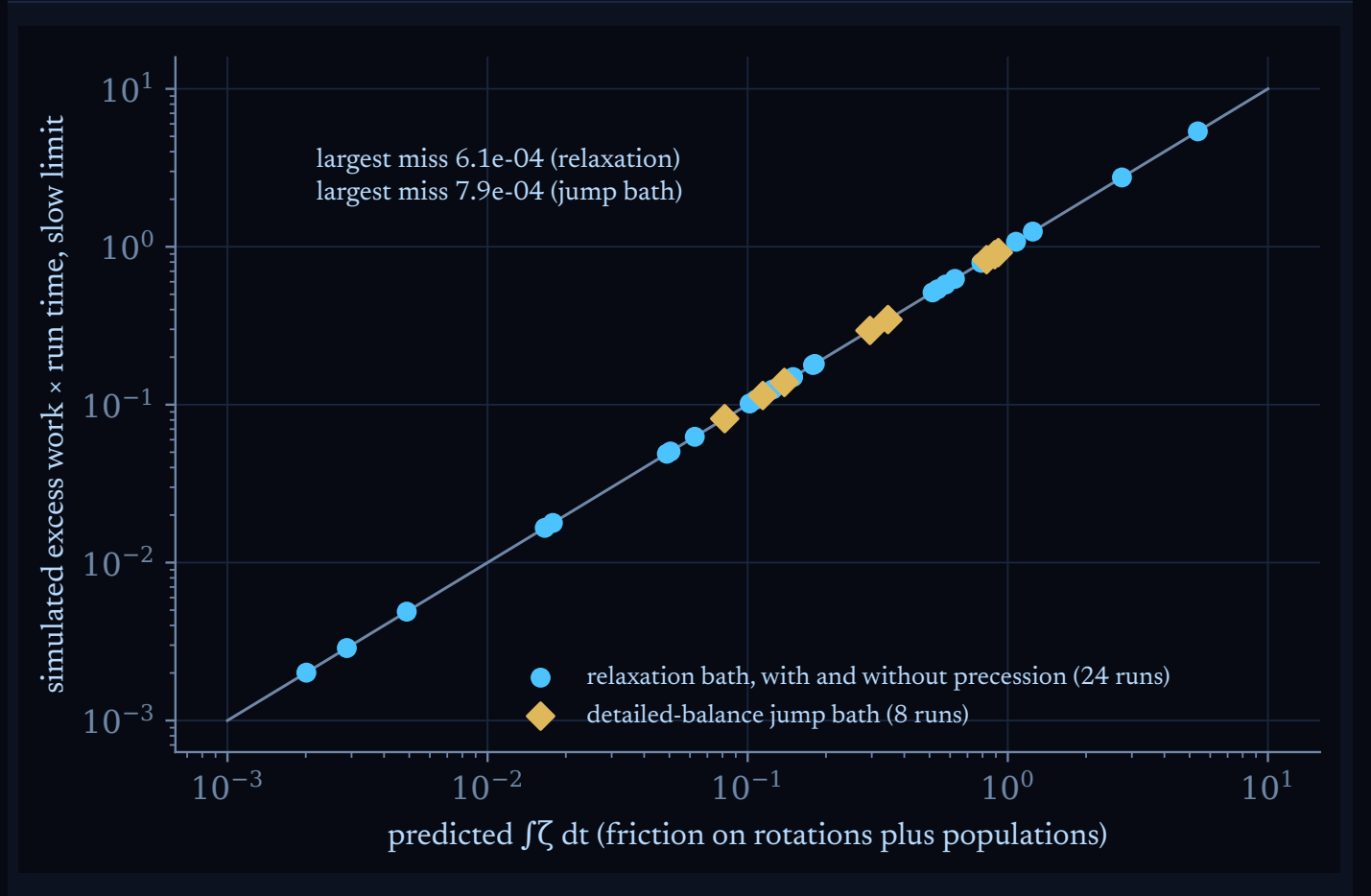
FIGURE 5. Friction on projector rotations, tested. Each point is one exact simulation of a slowly driven system in contact with a bath, taken to the slow limit from four run lengths, against the prediction \int \zeta dt . Circles: the relaxation bath, with and without precession. Diamonds: a detailed-balance jump bath the law was not built on.
