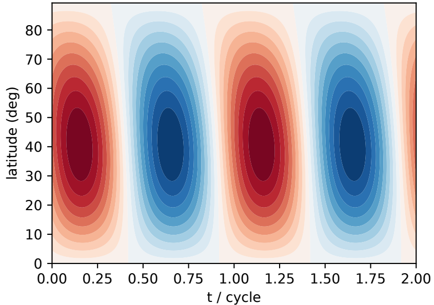
G=-1 : equatorward (solar-like)
