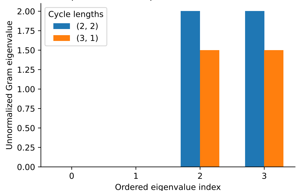
D. Equal normalized profiles hide different scales
