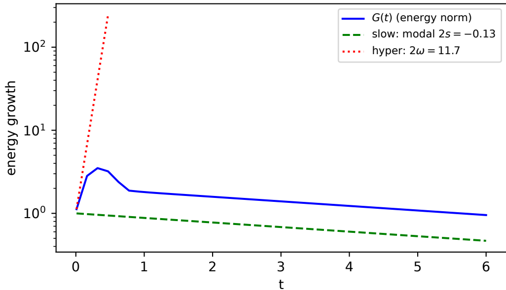
The hair ladder at 0.9 \alpha_{0c} : three computed rates
