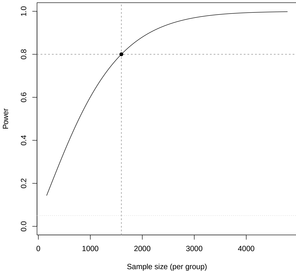
Power curve for DiD proportions
