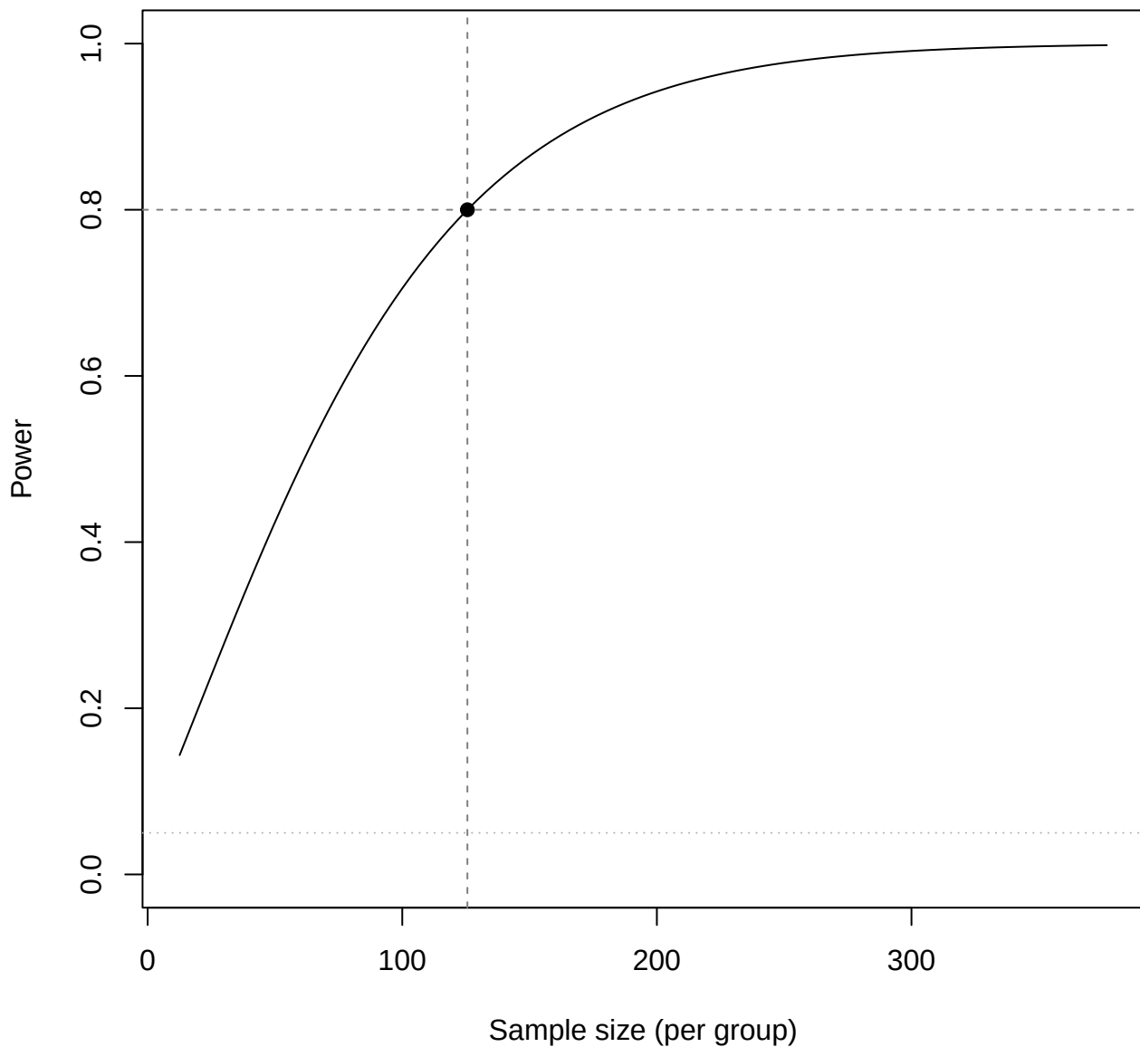
Power curve for DiD means
