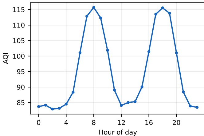
(a) Mean AQI by hour
