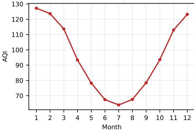
(b) Mean AQI by month
