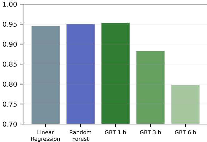
(b) Test R^2 (higher is better)
