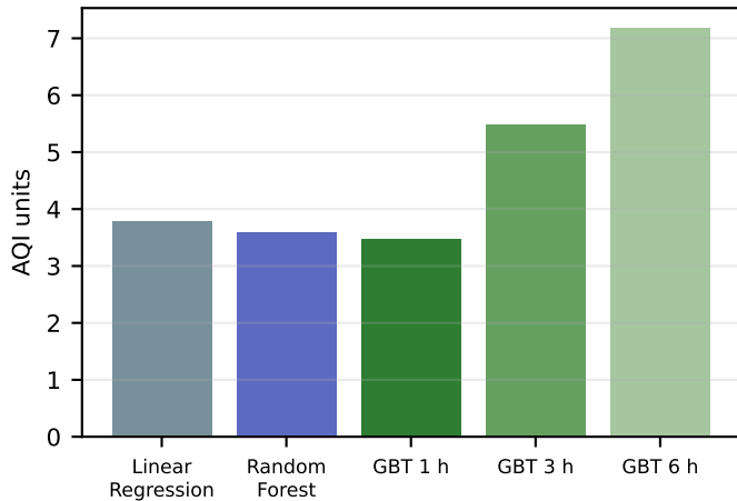
(a) Test RMSE (lower is better)
