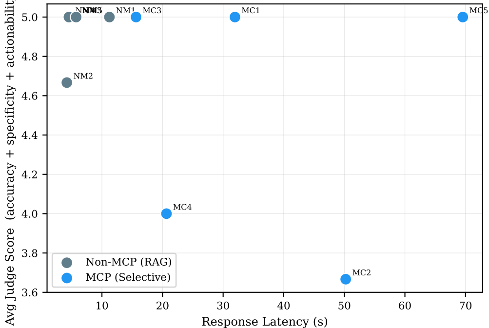
Latency vs Response Quality Trade-off (each point = one arm of one question)
