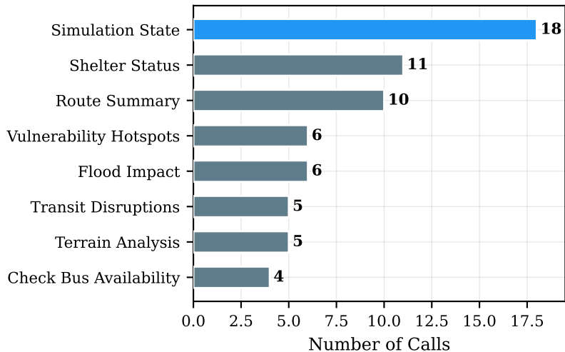
Most Frequently Called MCP Tools
