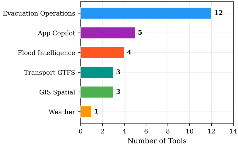
Tool Distribution Across MCP Servers
