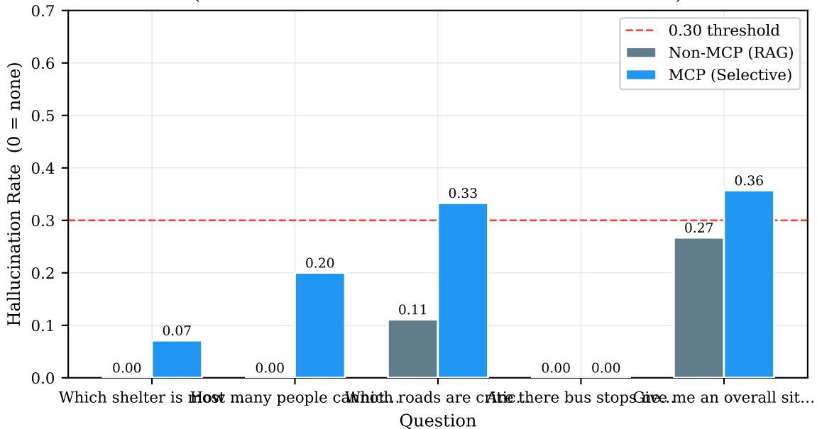
Hallucination Rate: Non-MCP vs MCP (fraction of numeric claims unverifiable in context)
