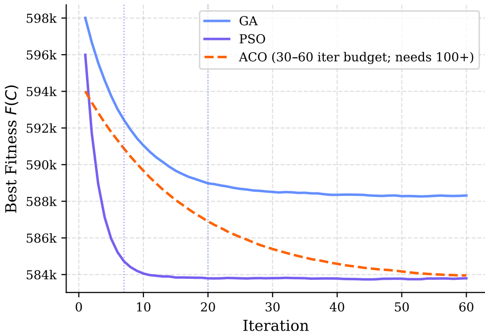
Convergence Curves — GA, ACO, PSO (Simulated; 60-iteration budget)
