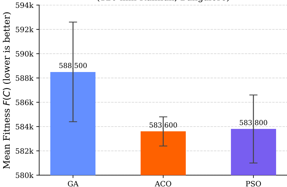
Algorithm Mean Fitness — 3-Run Stability Trial (120 mm Rainfall, Bangalore)
