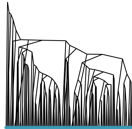
(a) Single linkage dendrogram
