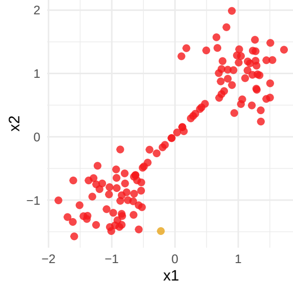
(f) Two-cluster solution
