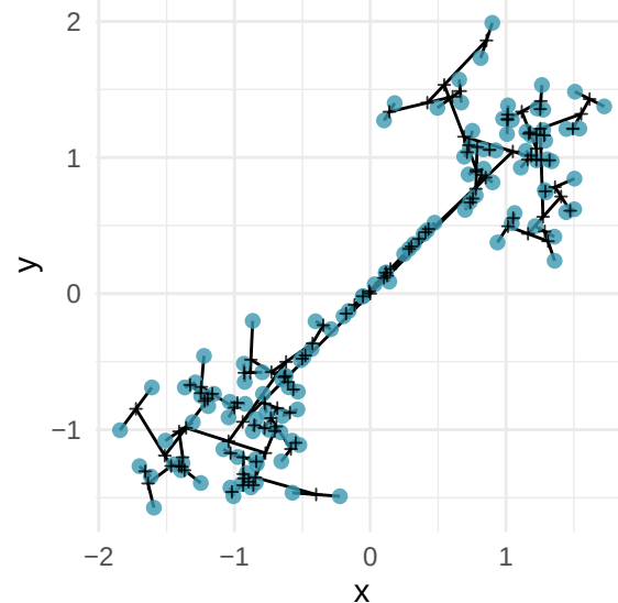
(e) Dendrogram in data space
