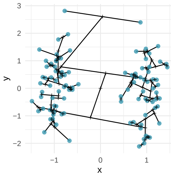
(e) Dendrogram in data space
