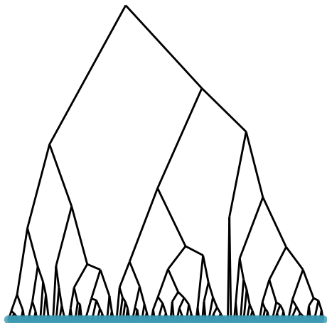
(a) Complete linkage dendrogram
