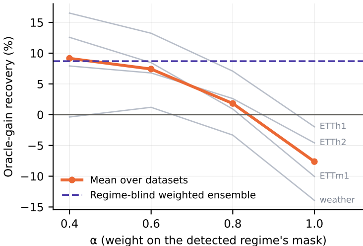
Trusting the regime label less helps more
