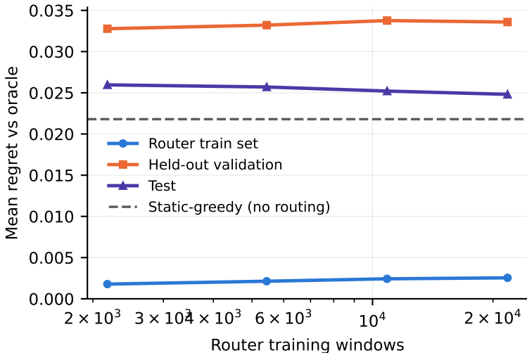
Routers memorize but never generalize
