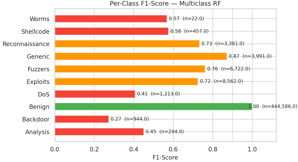
Figure 4: Per-class F1-scores for the multiclass Random Forest. Green bars ( \geq 0.90 ) indicate well-detected classes; orange bars (0.60–0.90) indicate moderate performance; red bars ( < 0.60 ) indicate rare classes suffering from insufficient training samples.
