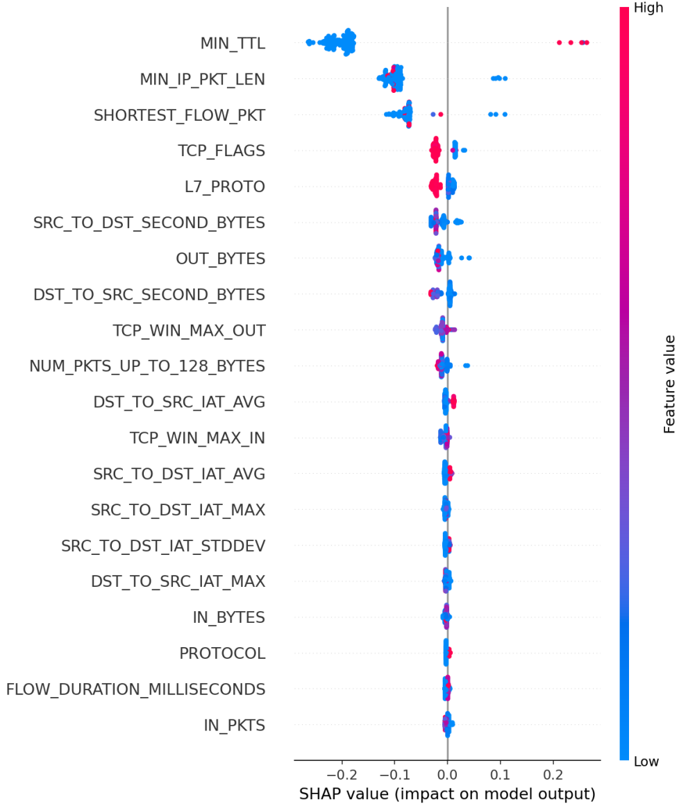
Figure 6: SHAP beeswarm plot showing the distribution and direction of feature impacts across 200 test samples. Each point is one flow; colour indicates feature value (red = high, blue = low). Features sorted by mean |\phi_j| .
