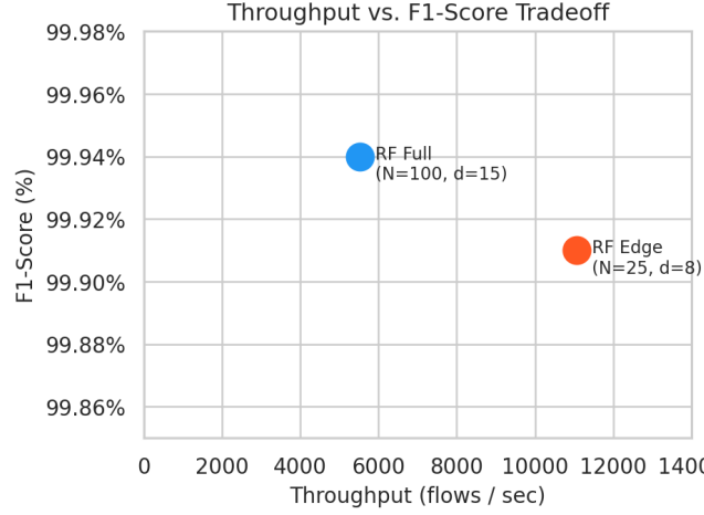
Figure 7: Throughput vs. F1-score tradeoff between the full and edge-optimised models. The edge model doubles throughput with negligible accuracy loss.
