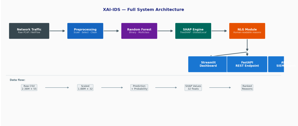
Figure 4: XAI-IDS full system architecture. Raw network traffic flows through preprocessing, Random Forest classification, SHAP attribution, and NLG to produce human-readable alerts delivered via the Streamlit dashboard, FastAPI endpoint, or SIEM export.
