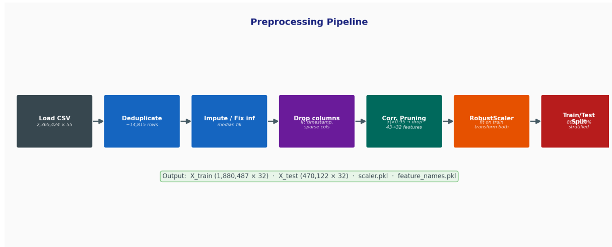
Figure 3: Preprocessing pipeline: seven sequential transformations reduce the raw 2.36\text{M} \times 55 dataset to clean 1.88\text{M} \times 32 training and 470\text{K} \times 32 test arrays saved as compressed .npz artefacts.
