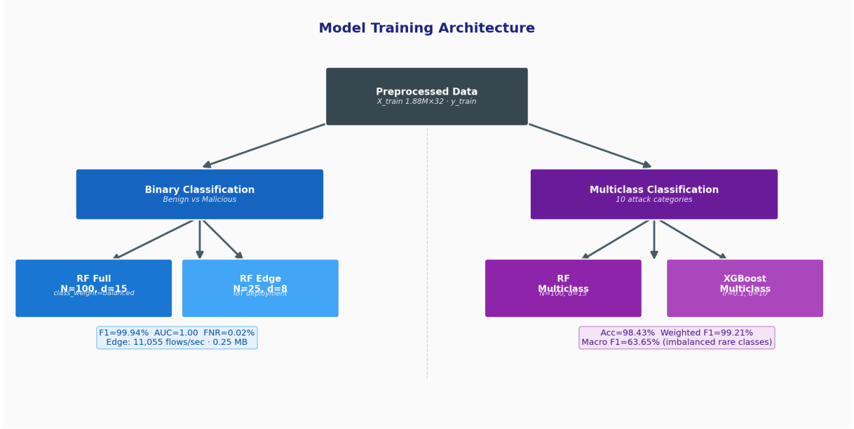
Figure 5: Training architecture. The preprocessed dataset feeds two parallel branches: binary classification (full and edge RF variants) and multiclass classification (RF and XGBoost). Achieved metrics are shown for each branch.
