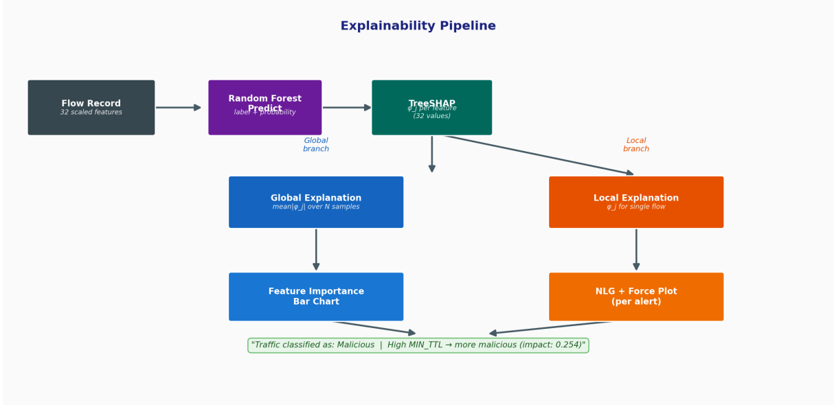
Figure 6: Explainability pipeline. Each prediction feeds into two branches: the global branch aggregates SHAP values across all samples for feature importance visualisation; the local branch produces per-alert force plots and NLG reasoning.
