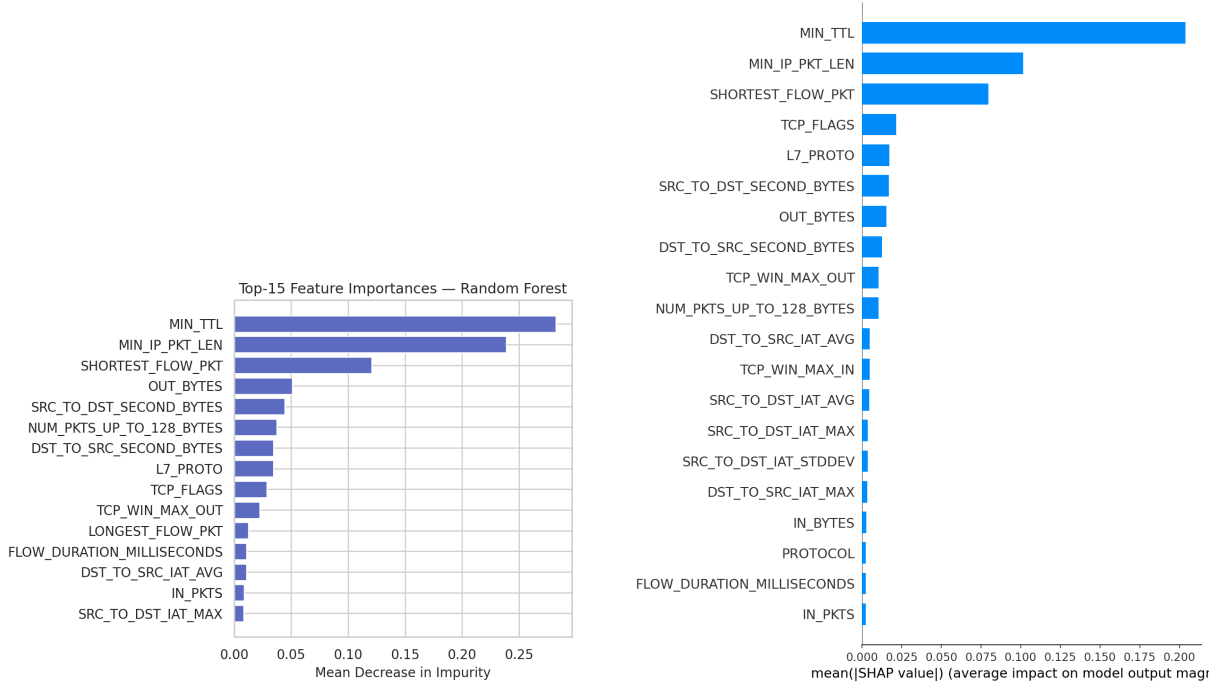
(a) Top-15 RF built-in feature importances (mean decrease in impurity).
