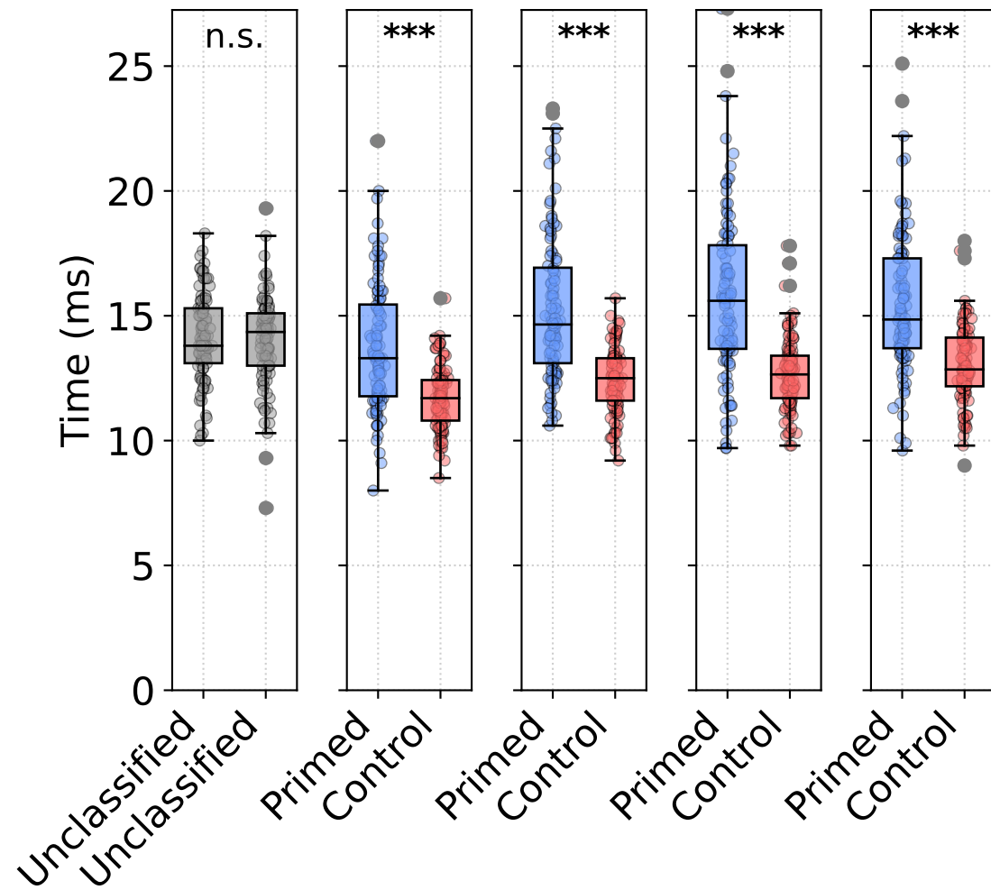
(b) Latency at 15% neuronal activation
