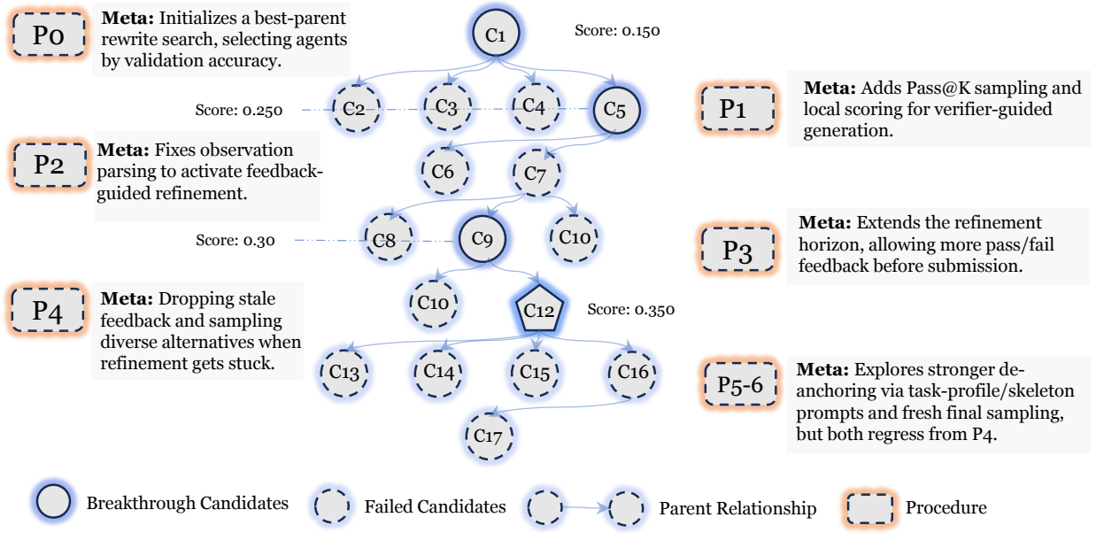
Figure 4 | Case study of procedure evolution on an ARC-AGI-2 task. Each P denotes a procedure produced or revised by the meta-agent, and each C denotes a candidate agent generated by the current procedure. Solid nodes are breakthrough candidates, dashed nodes are failed candidates, and arrows indicate parent relationships. The meta-agent improves the search process by changing the procedure across stages, while failed candidates provide feedback for later interventions.
