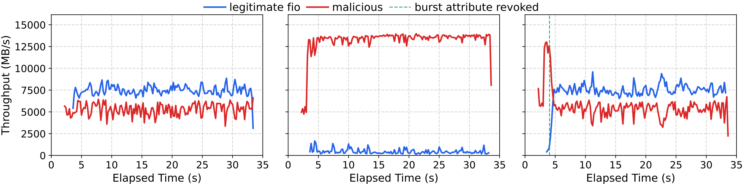
(a) Baseline: malicious no burst attribute
