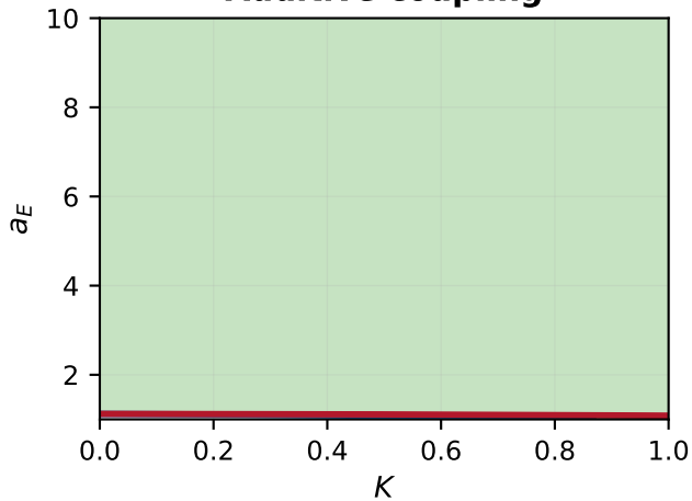
Additive coupling
