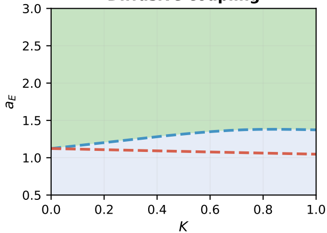
Diffusive coupling
