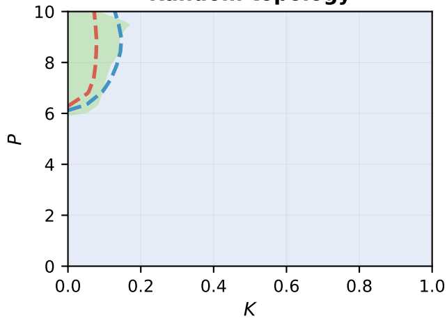
Random topology
