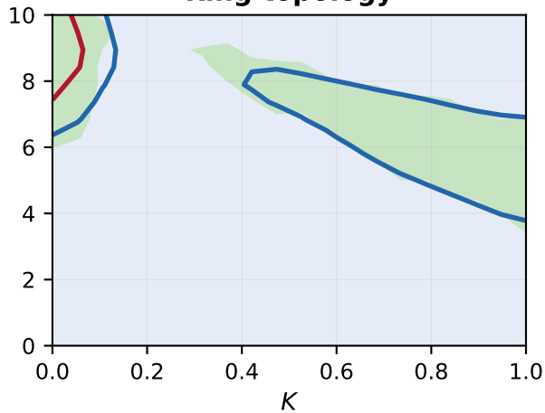
Ring topology
