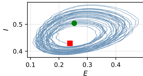
Phase portrait
