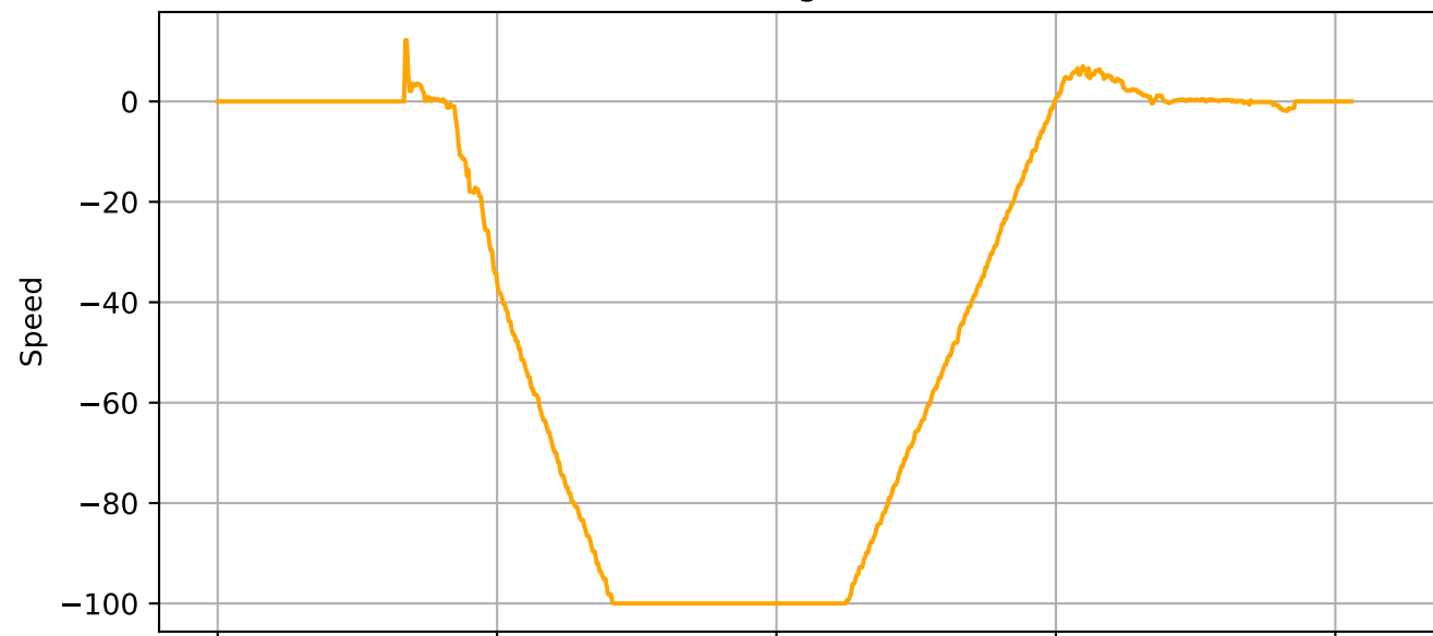
Integral Term (OFF - Windup Visibile)
