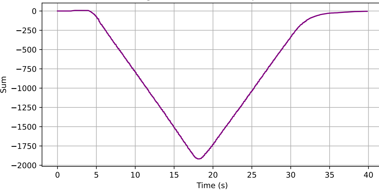
Integral Term (OFF - Windup Visibile)
