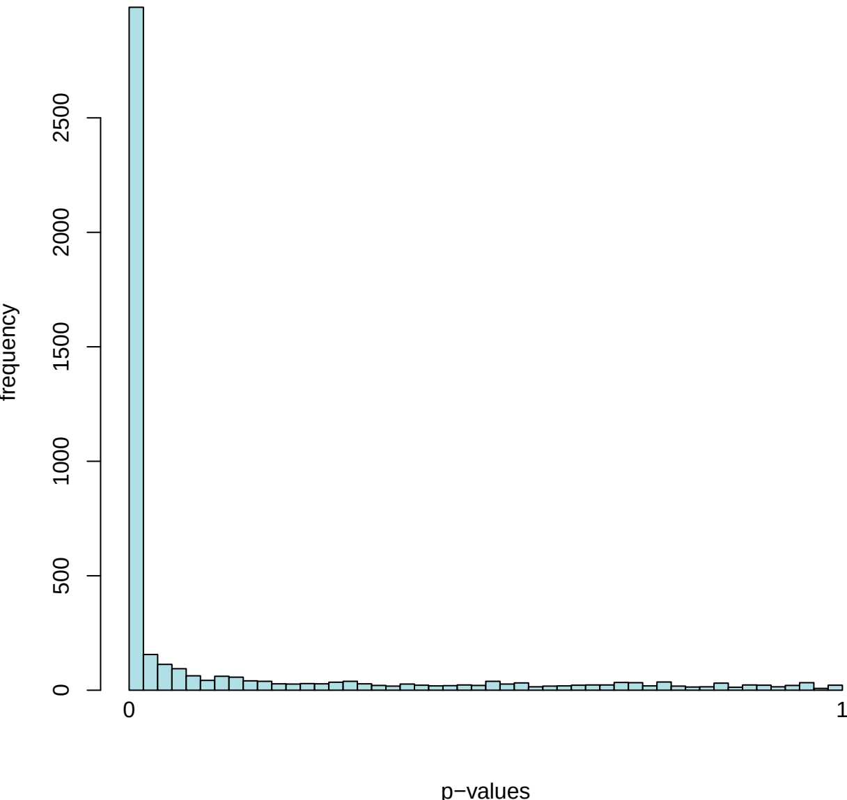
Histogram of p-values for Gene_Type: Wildtype vs Mutant
