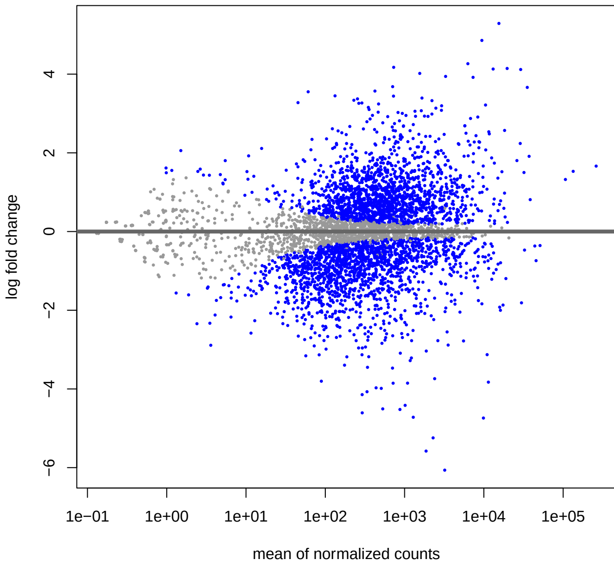
MA-plot for Gene_Type: Wildtype vs Mutant
