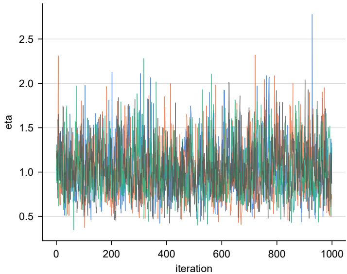
Censored GP
