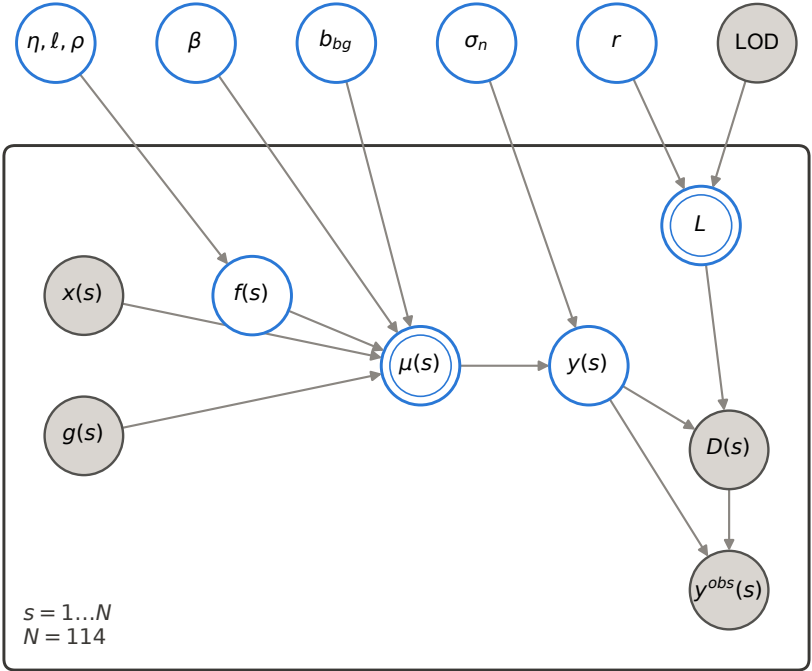
Plate diagram: six shared parameters, eight variables per each of the 114 locations
