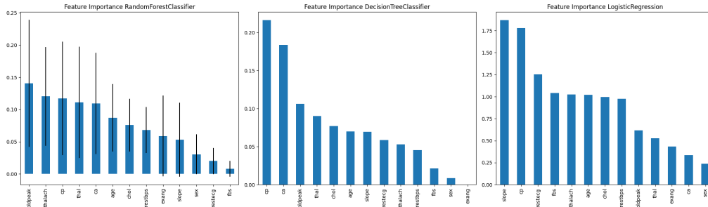
Figure 2. Feature Importance for the original version of the Health dataset
