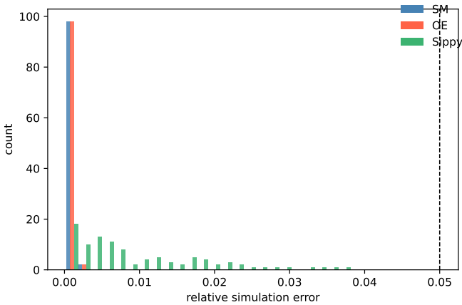
Fig. 1. Distribution of the relative simulation error for pysib SM, pysib OE, and SIPPY OE in the noisy-data comparison.
