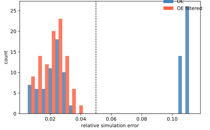
Fig. 3. Distribution of the relative simulation error for standard OE and filtered OE in the nonconvex benchmark.
