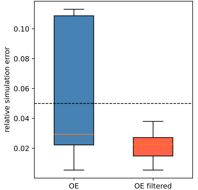
Fig. 4. Boxplot of the relative simulation error for the same methods.
