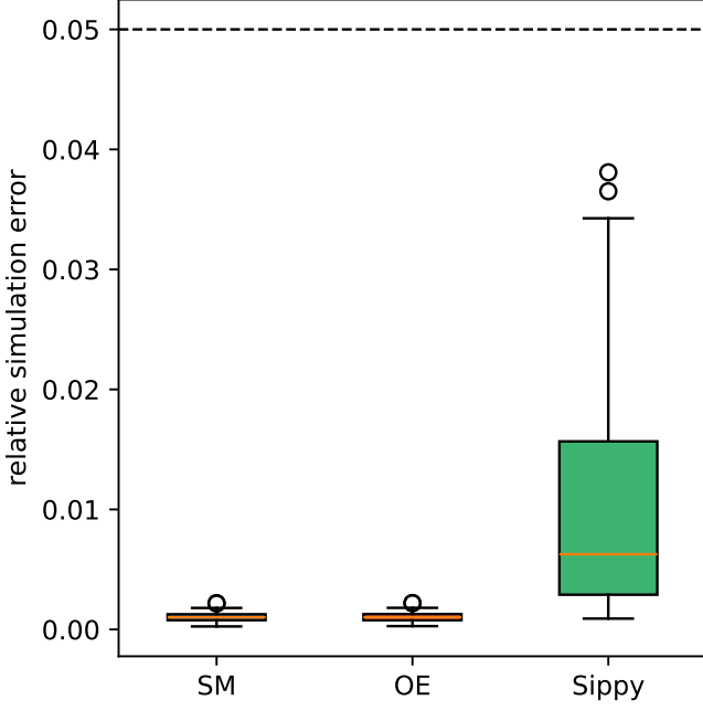
Fig. 2. Boxplot of the relative simulation error for the same methods.
