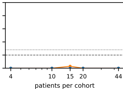
Boundary (saturated)
