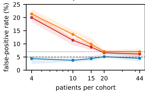
Spike-slab
