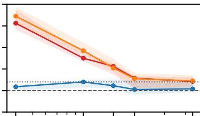
Skewed
