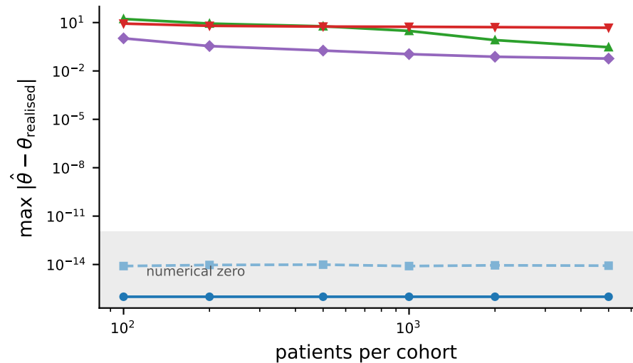
residual against the realised reference zero indicates functional reuse
