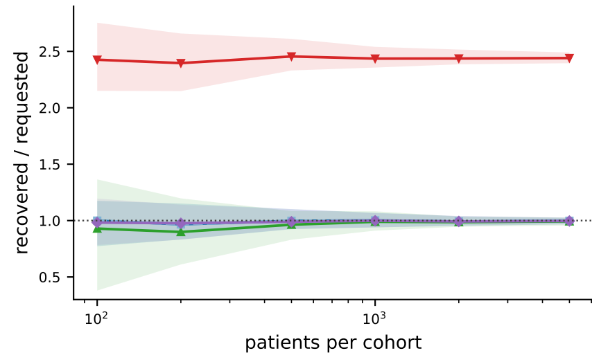
recovered / requested effect four of five estimators sit near 1
