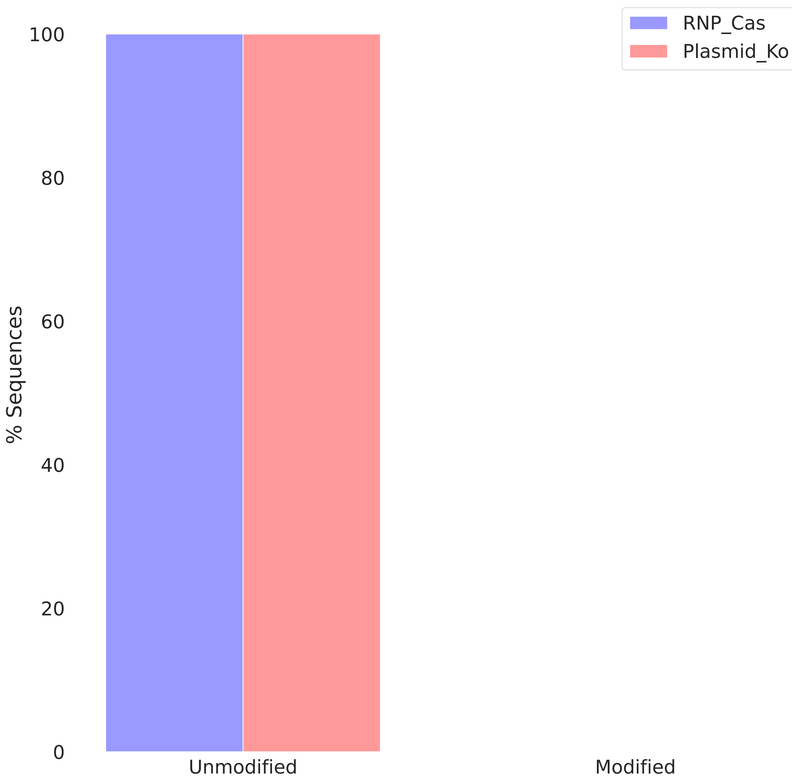
RNP_Cas VS Plasmid_Ko: bdnf_rc
