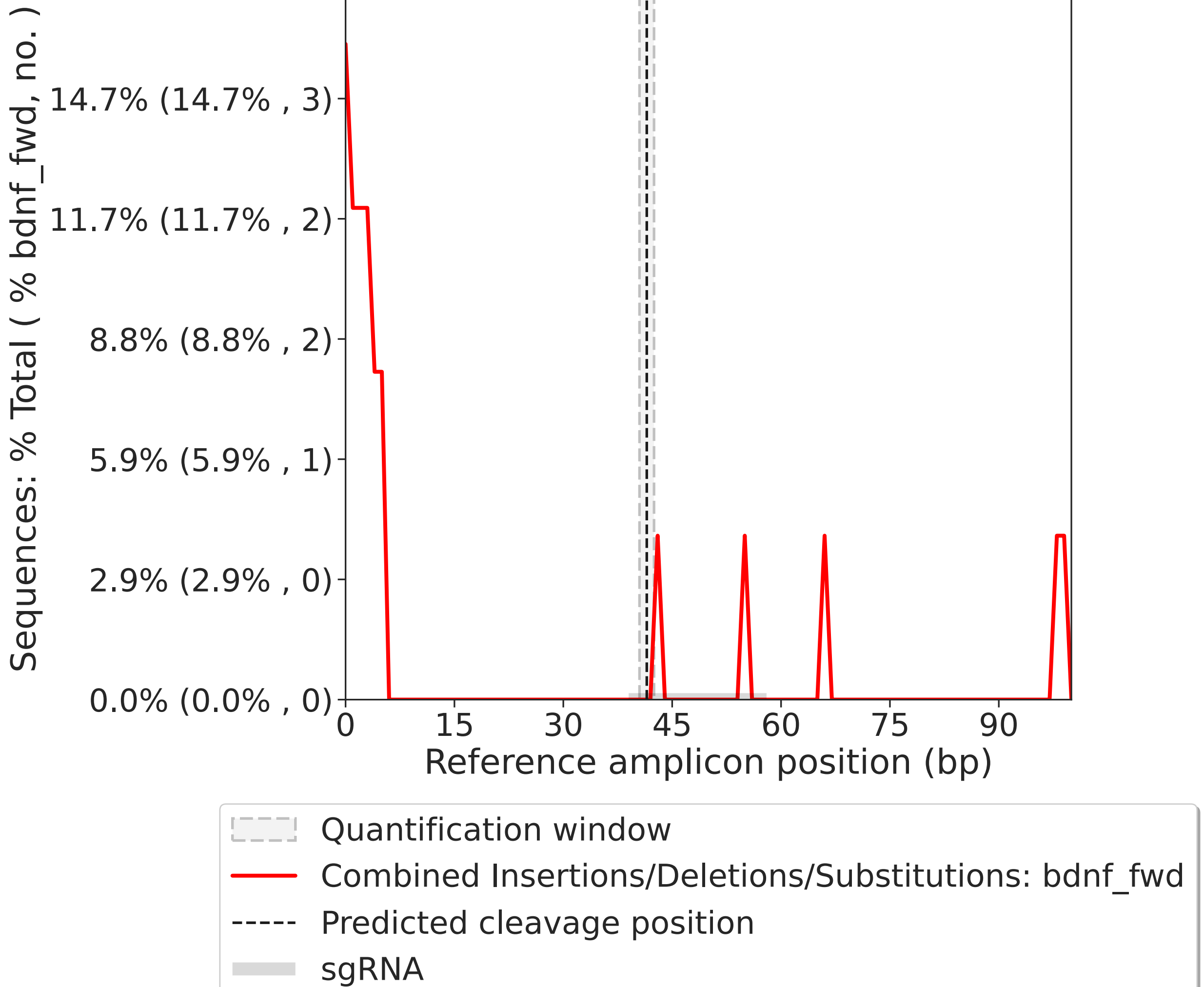
Mutation position distribution: bdnf_fwd
